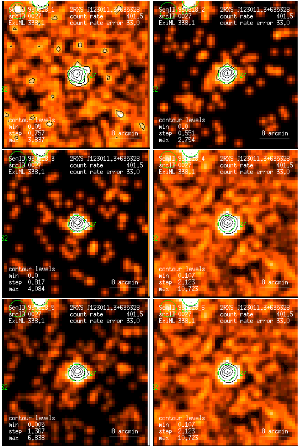
Figure 27: RASS 930618: detection 0027: band rate images, Gaussian filter: (1) PSPC channels 11 – 41, (2) 52 – 90, (3) 91 – 201, (4) 11 – 235, (5) 52 – 201, (6) 11 – 201. Broad band rates in counts/ks. Band rate contour levels in counts/ks/arcmin 2 .
