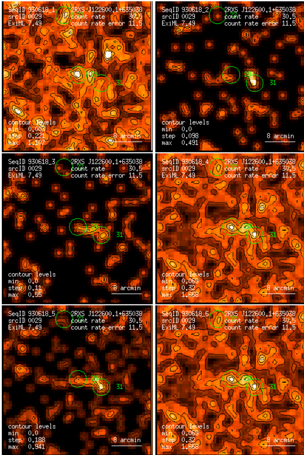
Figure 29: RASS 930618: detection 0029: band rate images, Gaussian filter: (1) PSPC channels 11 – 41, (2) 52 – 90, (3) 91 – 201, (4) 11 – 235, (5) 52 – 201, (6) 11 – 201. Broad band rates in counts/ks. Band rate contour levels in counts/ks/arcmin 2 .
