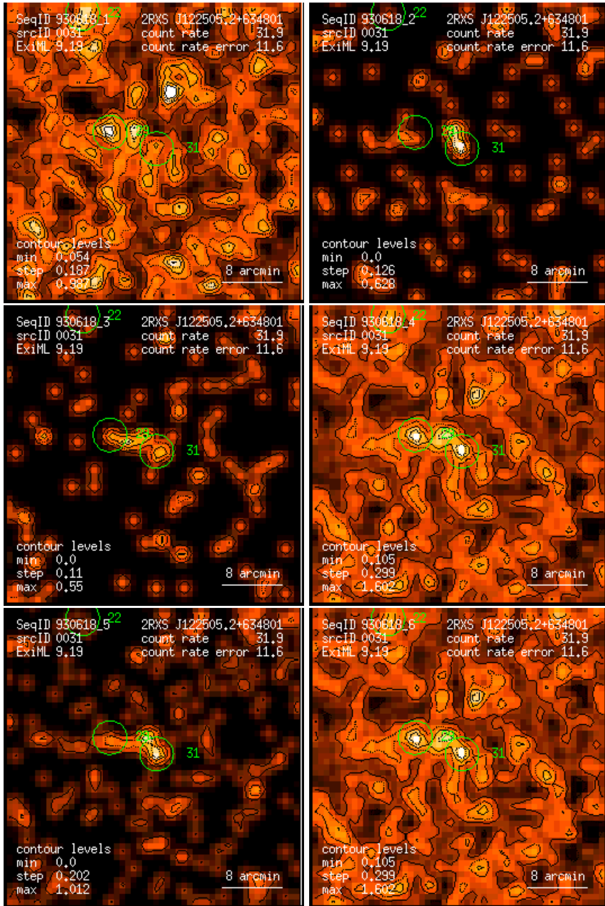
Figure 31: RASS 930618: detection 0031: band rate images, Gaussian filter: (1) PSPC channels 11 – 41, (2) 52 – 90, (3) 91 – 201, (4) 11 – 235, (5) 52 – 201, (6) 11 – 201. Broad band rates in counts/ks. Band rate contour levels in counts/ks/arcmin 2 .
