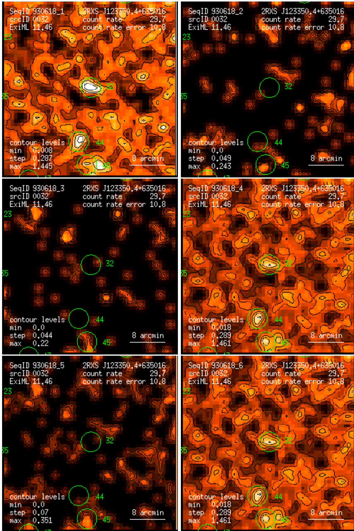
Figure 32: RASS 930618: detection 0032: band rate images, Gaussian filter: (1) PSPC channels 11 – 41, (2) 52 – 90, (3) 91 – 201, (4) 11 – 235, (5) 52 – 201, (6) 11 – 201. Broad band rates in counts/ks. Band rate contour levels in counts/ks/arcmin 2 .
