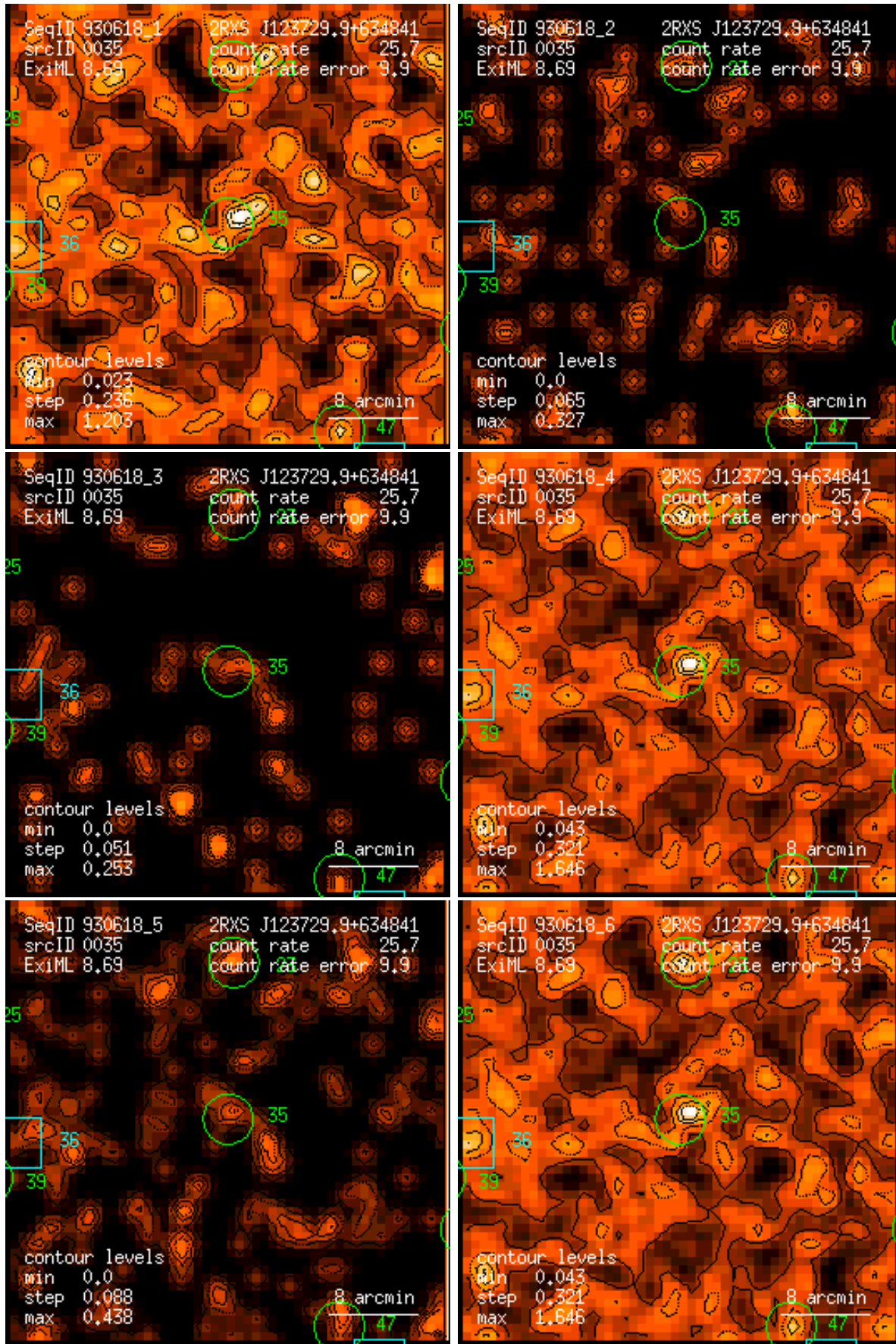
Figure 35: RASS 930618: detection 0035: band rate images, Gaussian filter: (1) PSPC channels 11 – 41, (2) 52 – 90, (3) 91 – 201, (4) 11 – 235, (5) 52 – 201, (6) 11 – 201. Broad band rates in counts/ks. Band rate contour levels in counts/ks/arcmin 2 .
