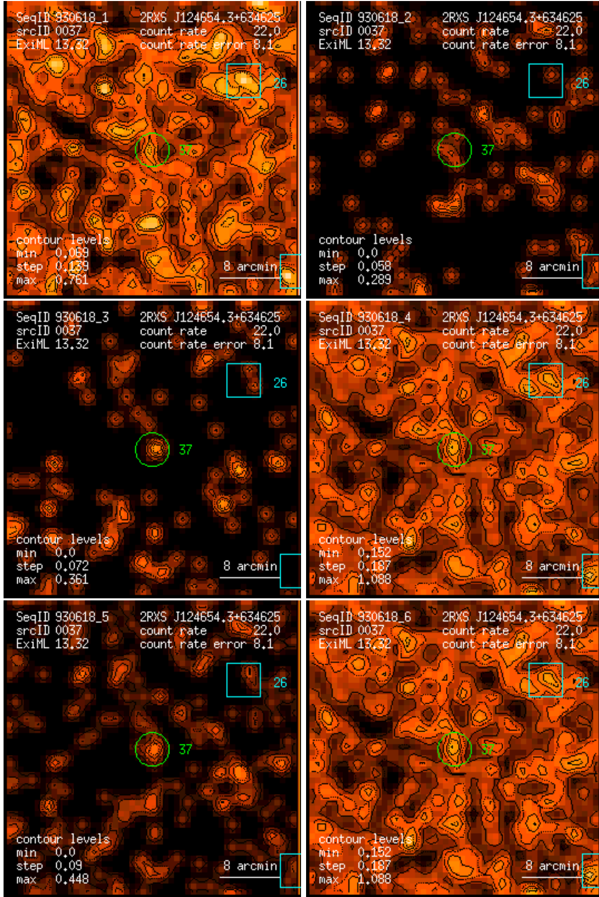
Figure 37: RASS 930618: detection 0037: band rate images, Gaussian filter: (1) PSPC channels 11 – 41, (2) 52 – 90, (3) 91 – 201, (4) 11 – 235, (5) 52 – 201, (6) 11 – 201. Broad band rates in counts/ks. Band rate contour levels in counts/ks/arcmin 2 .
