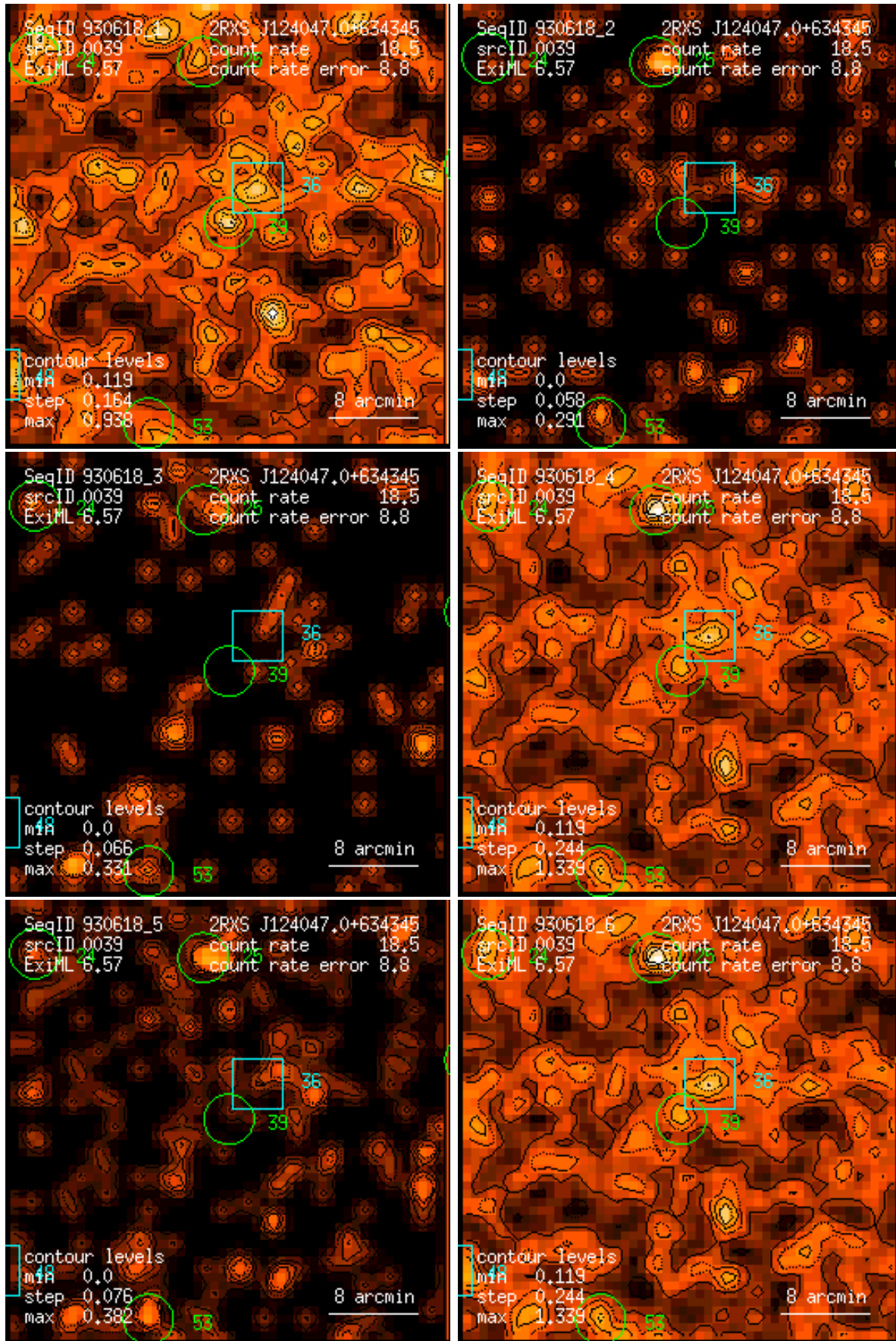
Figure 39: RASS 930618: detection 0039: band rate images, Gaussian filter: (1) PSPC channels 11 – 41, (2) 52 – 90, (3) 91 – 201, (4) 11 – 235, (5) 52 – 201, (6) 11 – 201. Broad band rates in counts/ks. Band rate contour levels in counts/ks/arcmin 2 .
