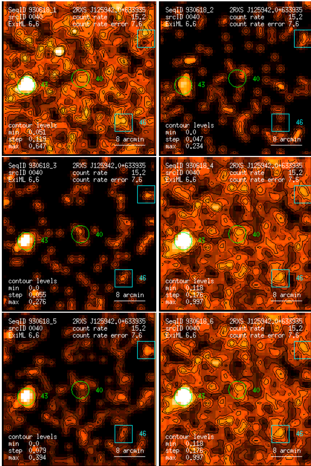
Figure 40: RASS 930618: detection 0040: band rate images, Gaussian filter: (1) PSPC channels 11 – 41, (2) 52 – 90, (3) 91 – 201, (4) 11 – 235, (5) 52 – 201, (6) 11 – 201. Broad band rates in counts/ks. Band rate contour levels in counts/ks/arcmin 2 .
