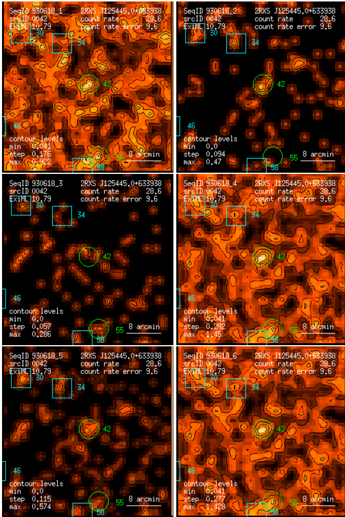
Figure 42: RASS 930618: detection 0042: band rate images, Gaussian filter: (1) PSPC channels 11 – 41, (2) 52 – 90, (3) 91 – 201, (4) 11 – 235, (5) 52 – 201, (6) 11 – 201. Broad band rates in counts/ks. Band rate contour levels in counts/ks/arcmin 2 .
