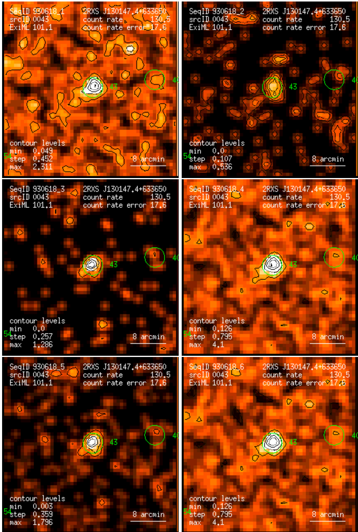
Figure 43: RASS 930618: detection 0043: band rate images, Gaussian filter: (1) PSPC channels 11 – 41, (2) 52 – 90, (3) 91 – 201, (4) 11 – 235, (5) 52 – 201, (6) 11 – 201. Broad band rates in counts/ks. Band rate contour levels in counts/ks/arcmin 2 .
