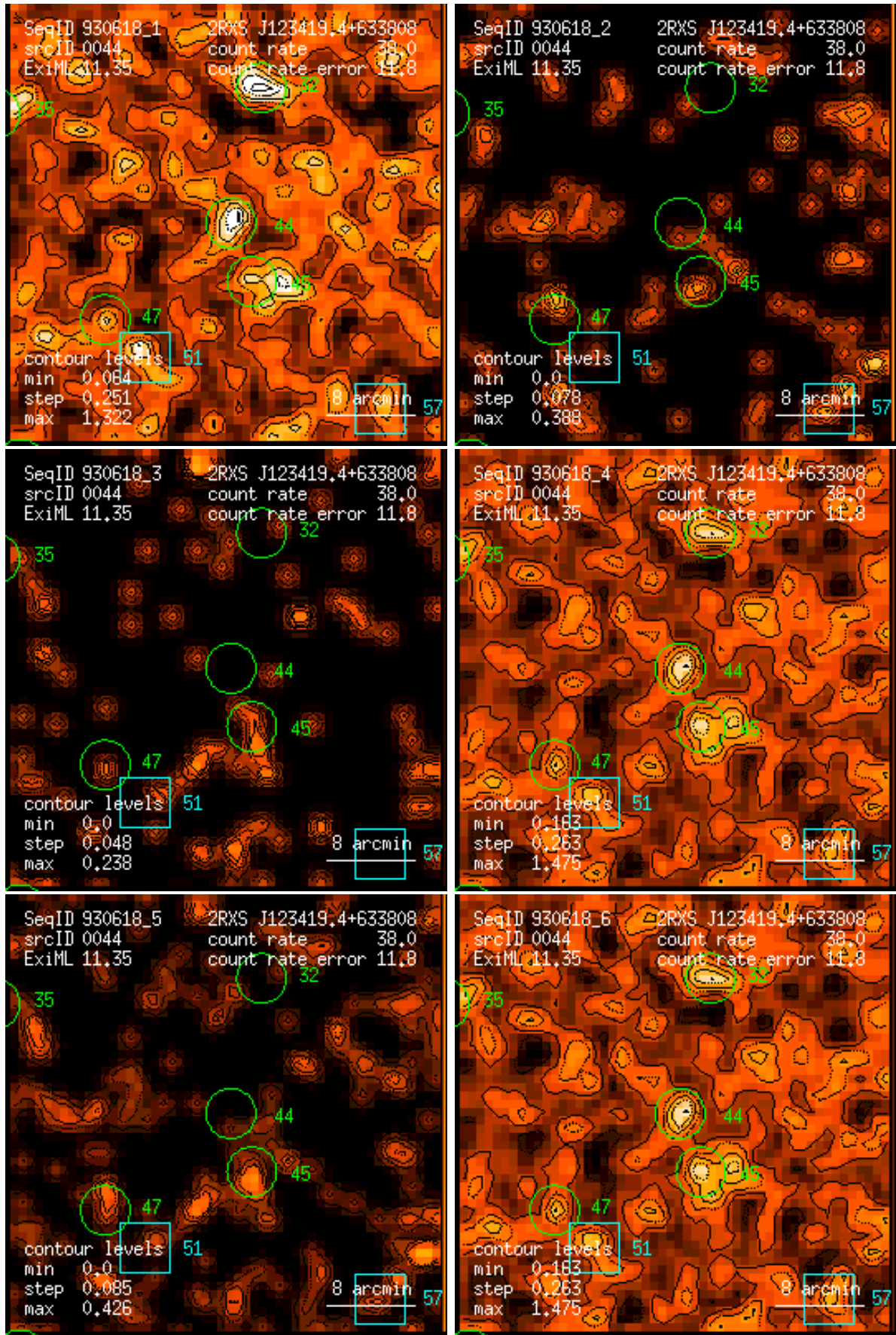
Figure 44: RASS 930618: detection 0044: band rate images, Gaussian filter: (1) PSPC channels 11 – 41, (2) 52 – 90, (3) 91 – 201, (4) 11 – 235, (5) 52 – 201, (6) 11 – 201. Broad band rates in counts/ks. Band rate contour levels in counts/ks/arcmin 2 .
