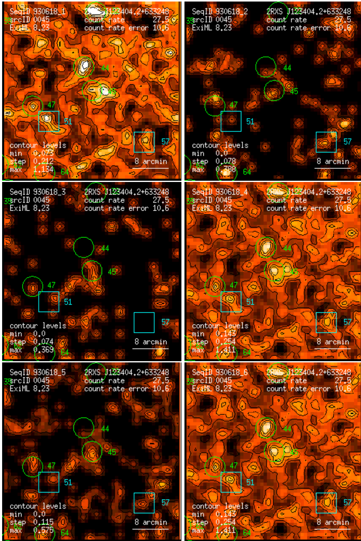
Figure 45: RASS 930618: detection 0045: band rate images, Gaussian filter: (1) PSPC channels 11 – 41, (2) 52 – 90, (3) 91 – 201, (4) 11 – 235, (5) 52 – 201, (6) 11 – 201. Broad band rates in counts/ks. Band rate contour levels in counts/ks/arcmin 2 .
