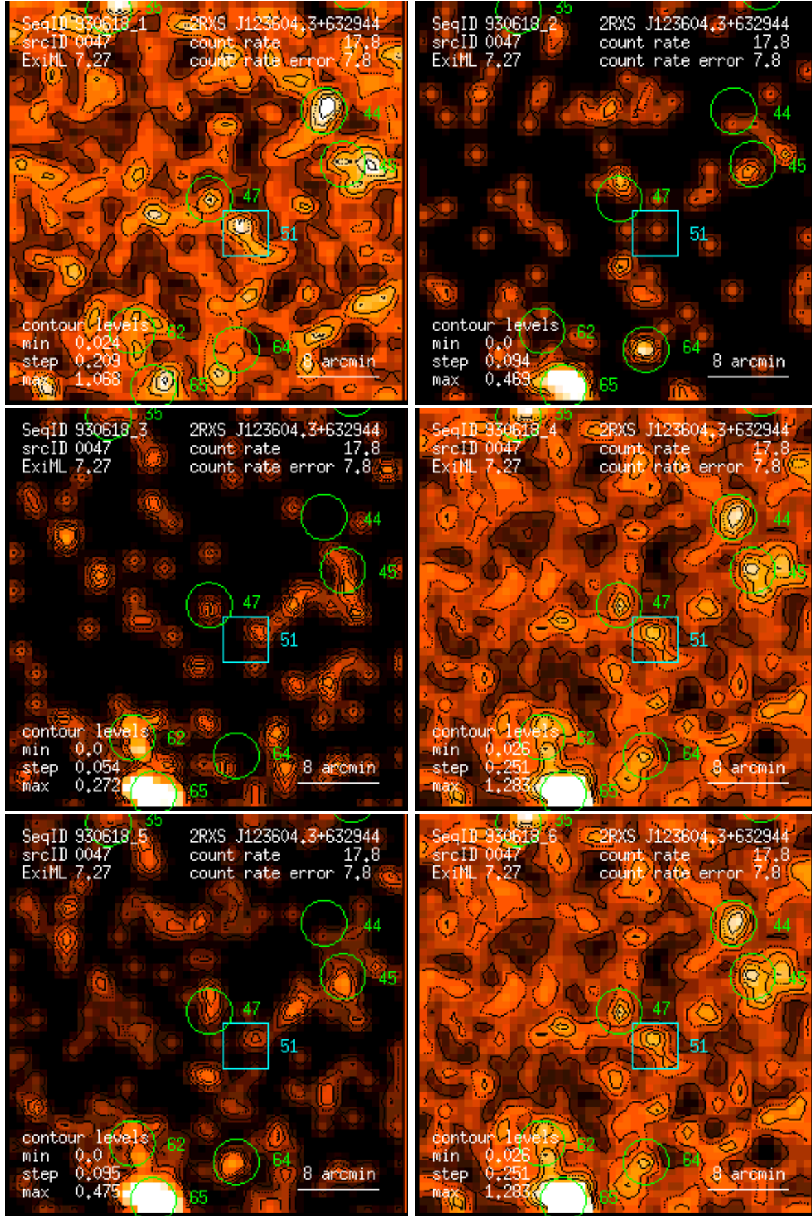
Figure 47: RASS 930618: detection 0047: band rate images, Gaussian filter: (1) PSPC channels 11 – 41, (2) 52 – 90, (3) 91 – 201, (4) 11 – 235, (5) 52 – 201, (6) 11 – 201. Broad band rates in counts/ks. Band rate contour levels in counts/ks/arcmin 2 .
