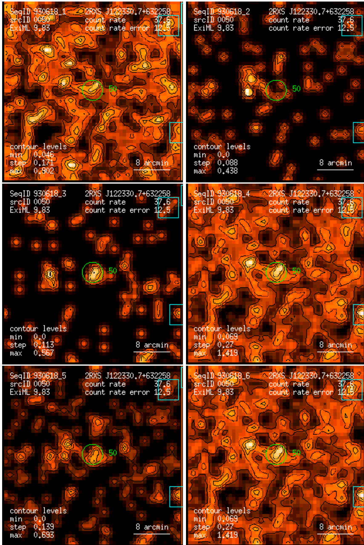
Figure 50: RASS 930618: detection 0050: band rate images, Gaussian filter: (1) PSPC channels 11 – 41, (2) 52 – 90, (3) 91 – 201, (4) 11 – 235, (5) 52 – 201, (6) 11 – 201. Broad band rates in counts/ks. Band rate contour levels in counts/ks/arcmin 2 .
