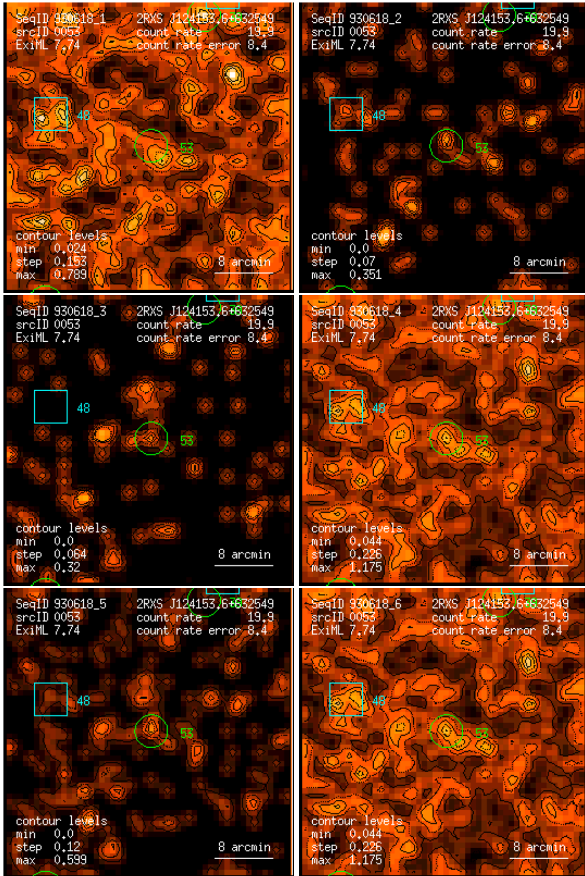
Figure 53: RASS 930618: detection 0053: band rate images, Gaussian filter: (1) PSPC channels 11 – 41, (2) 52 – 90, (3) 91 – 201, (4) 11 – 235, (5) 52 – 201, (6) 11 – 201. Broad band rates in counts/ks. Band rate contour levels in counts/ks/arcmin 2 .
