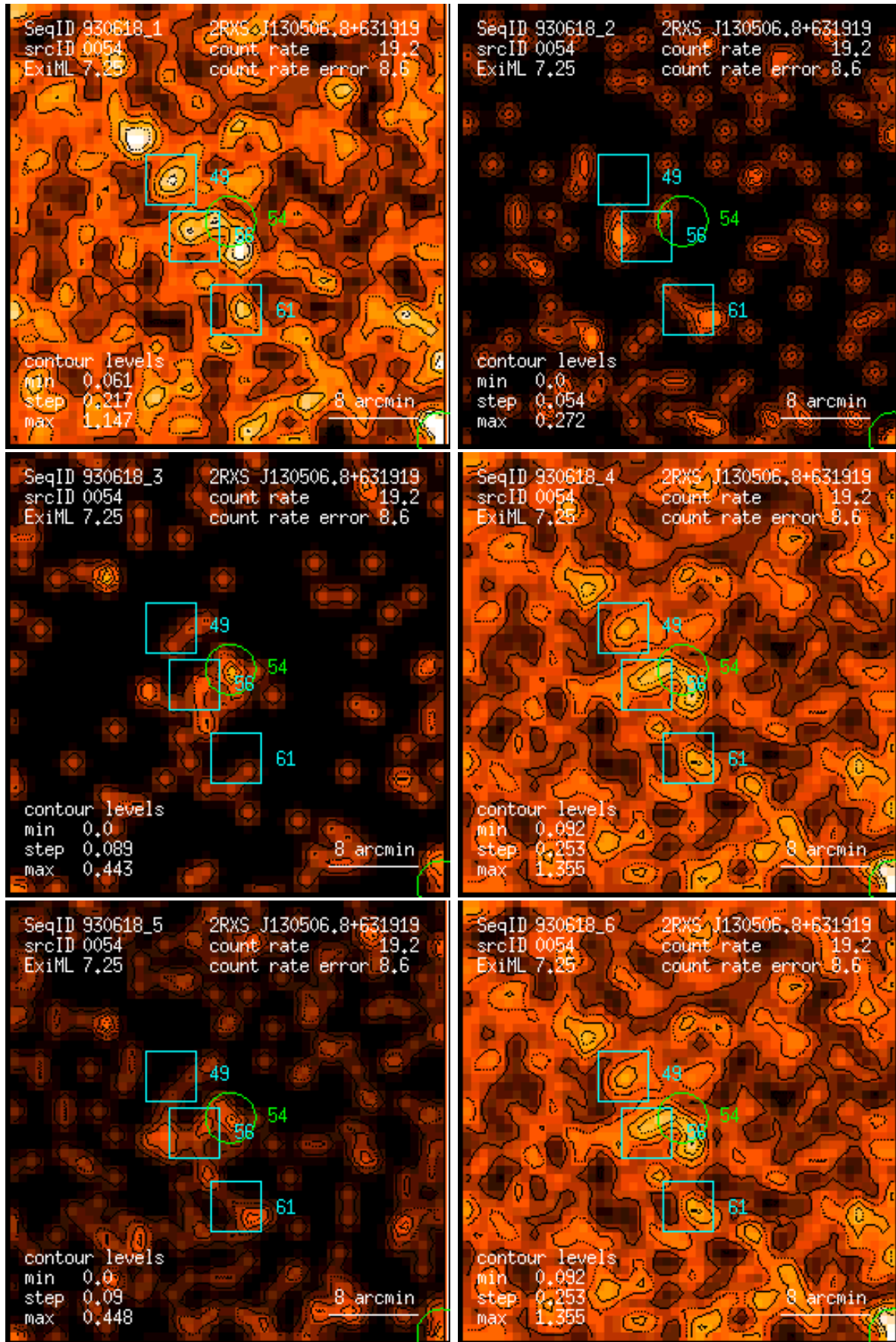
Figure 54: RASS 930618: detection 0054: band rate images, Gaussian filter: (1) PSPC channels 11 – 41, (2) 52 – 90, (3) 91 – 201, (4) 11 – 235, (5) 52 – 201, (6) 11 – 201. Broad band rates in counts/ks. Band rate contour levels in counts/ks/arcmin 2 .
