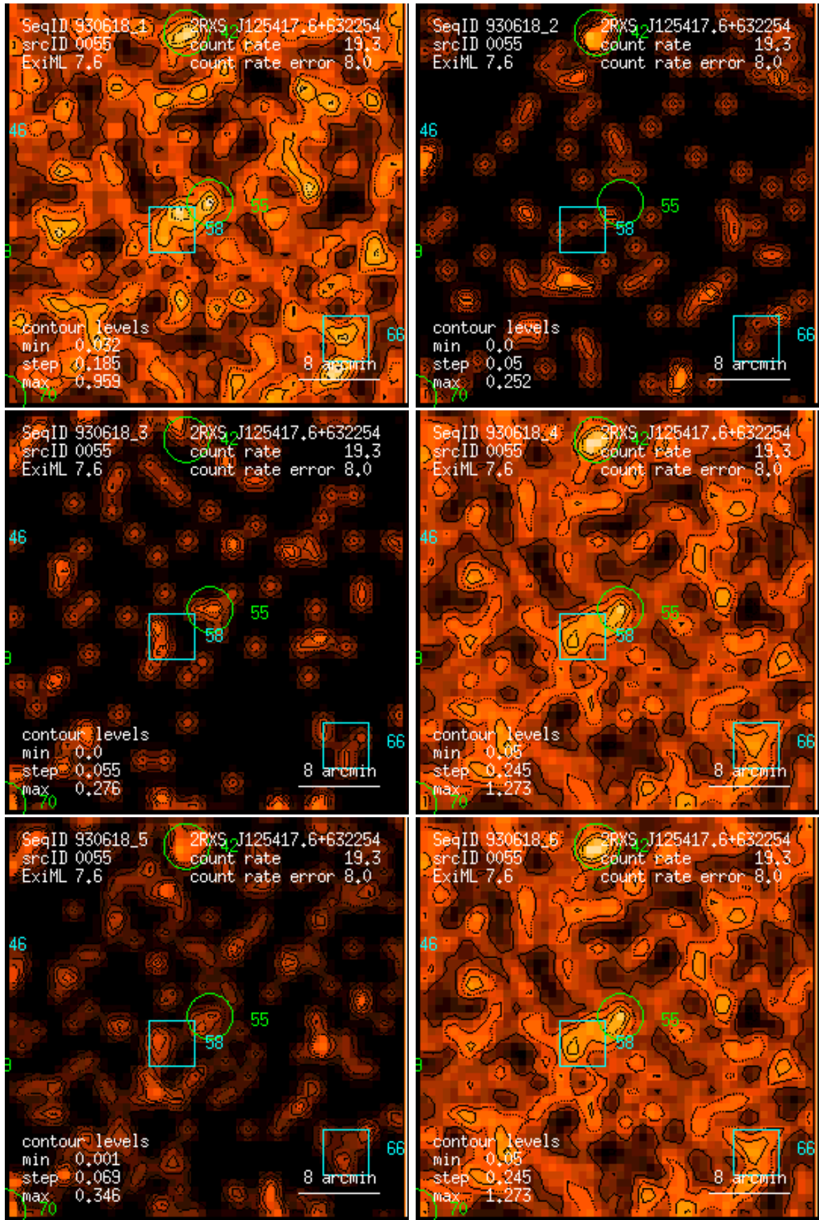
Figure 55: RASS 930618: detection 0055: band rate images, Gaussian filter: (1) PSPC channels 11 – 41, (2) 52 – 90, (3) 91 – 201, (4) 11 – 235, (5) 52 – 201, (6) 11 – 201. Broad band rates in counts/ks. Band rate contour levels in counts/ks/arcmin 2 .
