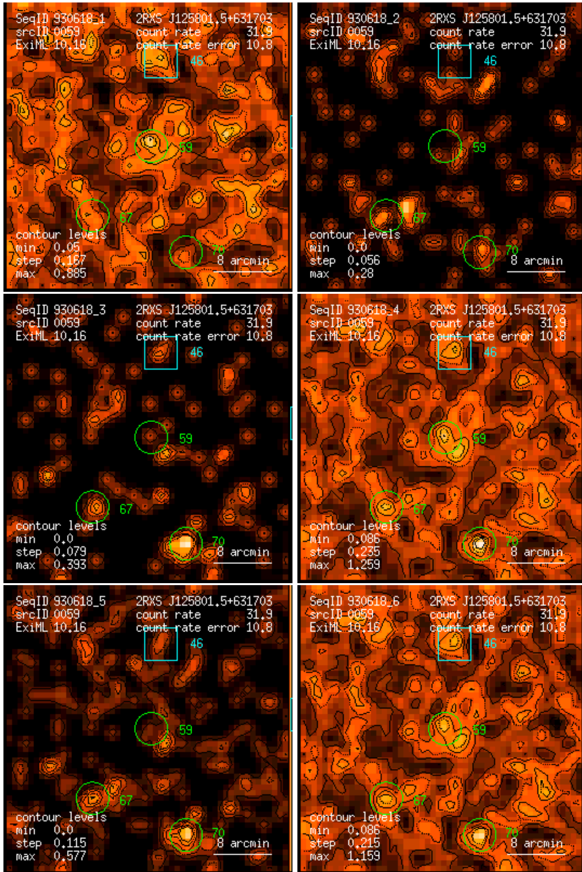
Figure 59: RASS 930618: detection 0059: band rate images, Gaussian filter: (1) PSPC channels 11 – 41, (2) 52 – 90, (3) 91 – 201, (4) 11 – 235, (5) 52 – 201, (6) 11 – 201. Broad band rates in counts/ks. Band rate contour levels in counts/ks/arcmin 2 .
