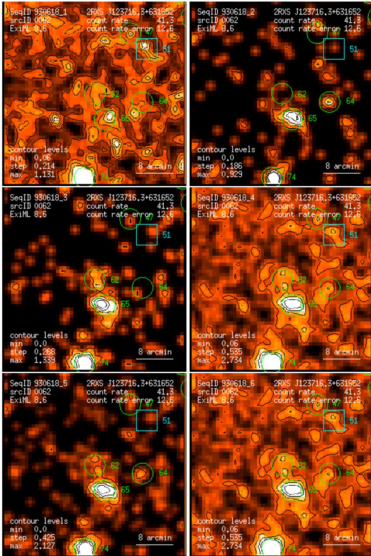
Figure 62: RASS 930618: detection 0062: band rate images, Gaussian filter: (1) PSPC channels 11 – 41, (2) 52 – 90, (3) 91 – 201, (4) 11 – 235, (5) 52 – 201, (6) 11 – 201. Broad band rates in counts/ks. Band rate contour levels in counts/ks/arcmin 2 .
