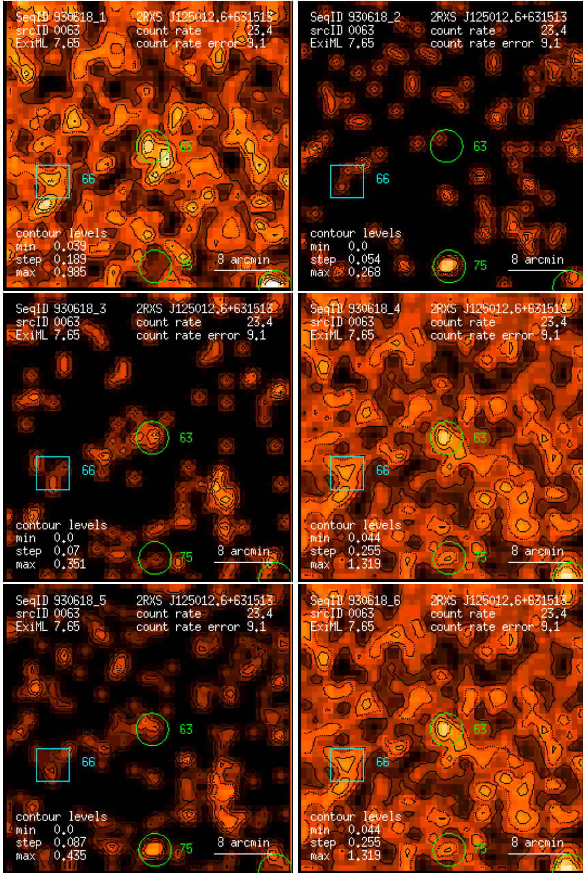
Figure 63: RASS 930618: detection 0063: band rate images, Gaussian filter: (1) PSPC channels 11 – 41, (2) 52 – 90, (3) 91 – 201, (4) 11 – 235, (5) 52 – 201, (6) 11 – 201. Broad band rates in counts/ks. Band rate contour levels in counts/ks/arcmin 2 .
