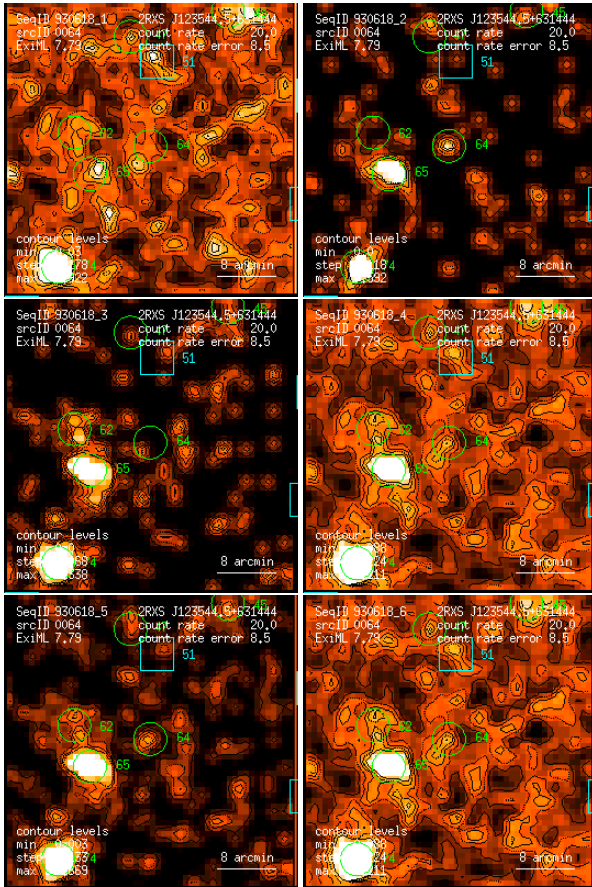
Figure 64: RASS 930618: detection 0064: band rate images, Gaussian filter: (1) PSPC channels 11 – 41, (2) 52 – 90, (3) 91 – 201, (4) 11 – 235, (5) 52 – 201, (6) 11 – 201. Broad band rates in counts/ks. Band rate contour levels in counts/ks/arcmin 2 .
