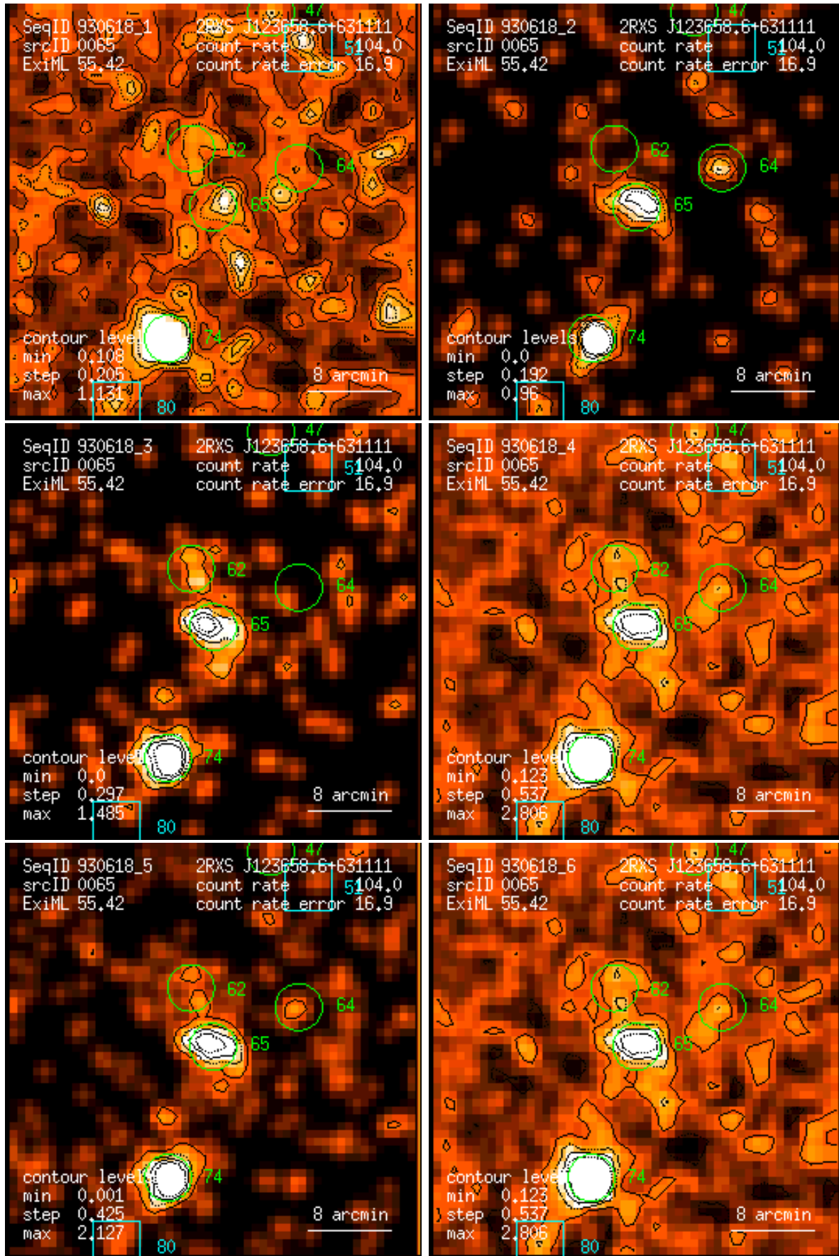
Figure 65: RASS 930618: detection 0065: band rate images, Gaussian filter: (1) PSPC channels 11 – 41, (2) 52 – 90, (3) 91 – 201, (4) 11 – 235, (5) 52 – 201, (6) 11 – 201. Broad band rates in counts/ks. Band rate contour levels in counts/ks/arcmin 2 .
