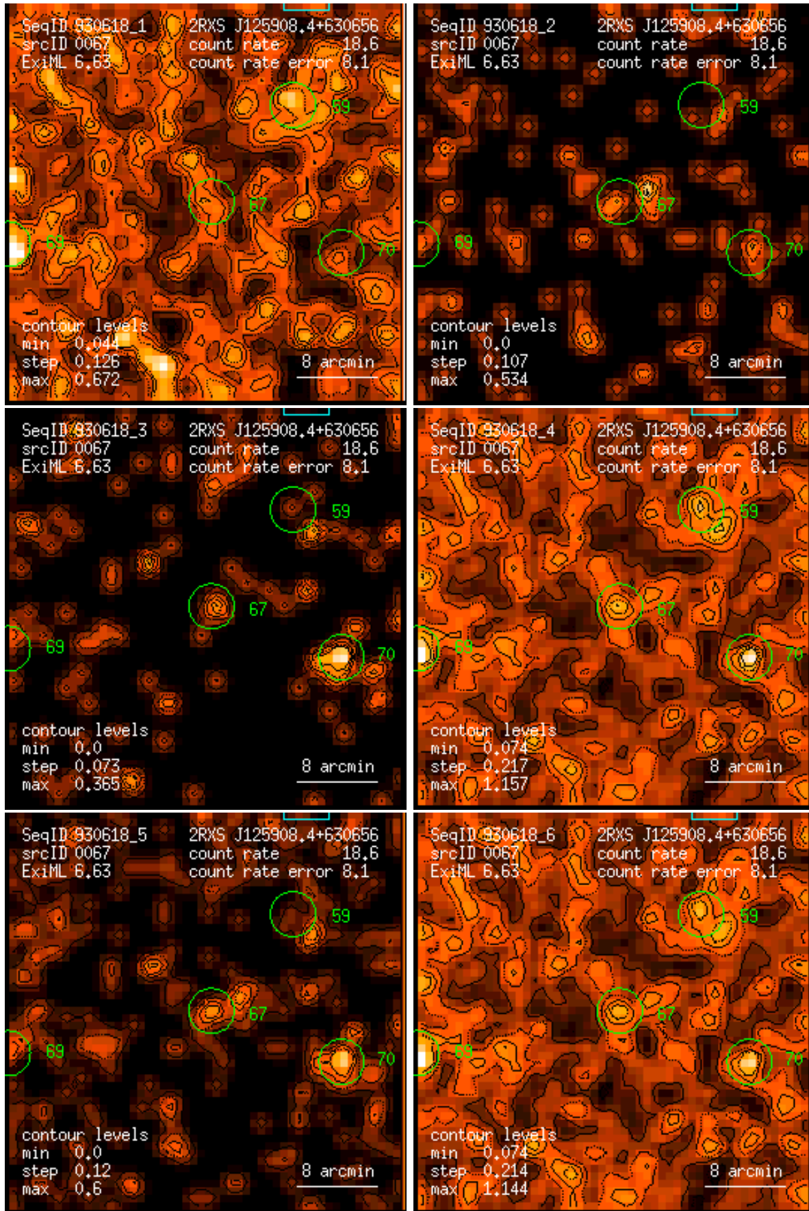
Figure 67: RASS 930618: detection 0067: band rate images, Gaussian filter: (1) PSPC channels 11 – 41, (2) 52 – 90, (3) 91 – 201, (4) 11 – 235, (5) 52 – 201, (6) 11 – 201. Broad band rates in counts/ks. Band rate contour levels in counts/ks/arcmin 2 .
