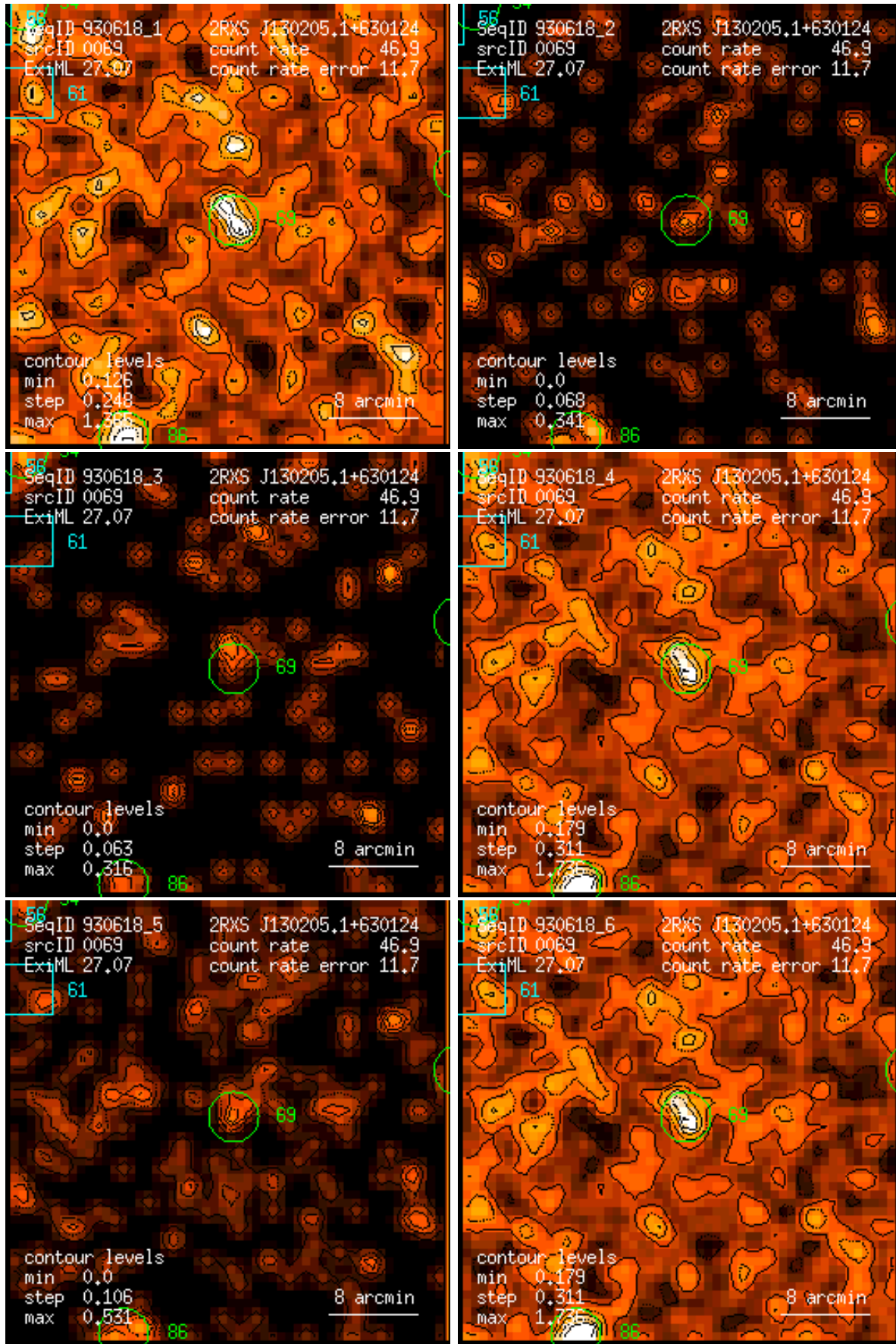
Figure 69: RASS 930618: detection 0069: band rate images, Gaussian filter: (1) PSPC channels 11 – 41, (2) 52 – 90, (3) 91 – 201, (4) 11 – 235, (5) 52 – 201, (6) 11 – 201. Broad band rates in counts/ks. Band rate contour levels in counts/ks/arcmin 2 .
