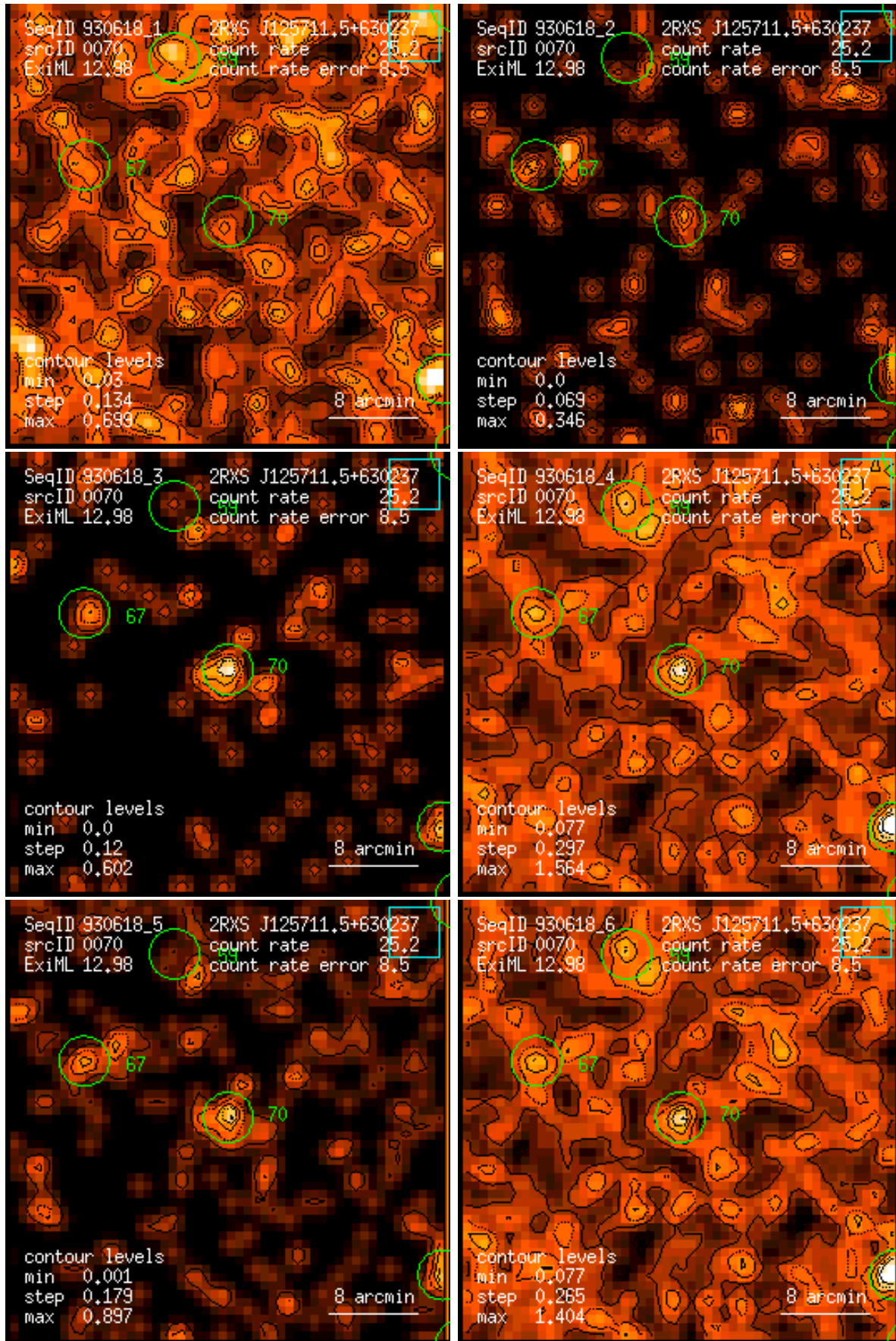
Figure 70: RASS 930618: detection 0070: band rate images, Gaussian filter: (1) PSPC channels 11 – 41, (2) 52 – 90, (3) 91 – 201, (4) 11 – 235, (5) 52 – 201, (6) 11 – 201. Broad band rates in counts/ks. Band rate contour levels in counts/ks/arcmin 2 .
