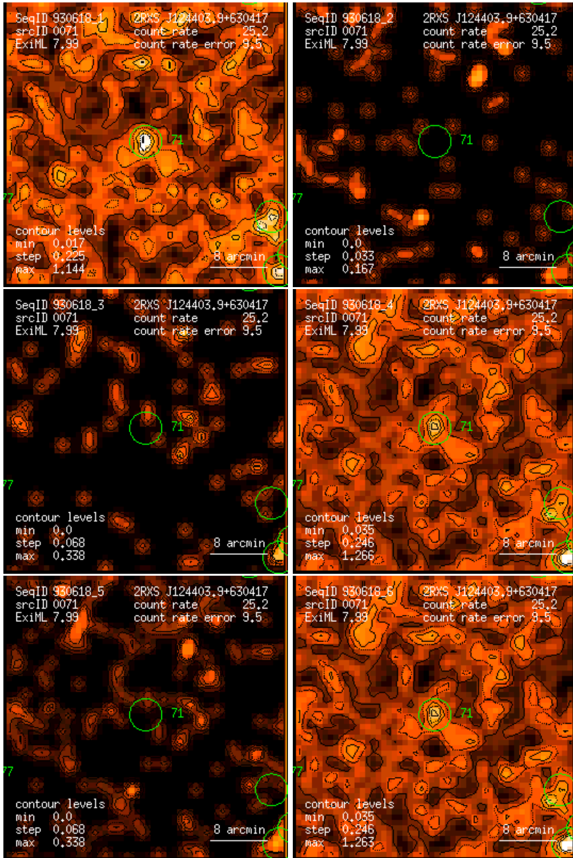
Figure 71: RASS 930618: detection 0071: band rate images, Gaussian filter: (1) PSPC channels 11 – 41, (2) 52 – 90, (3) 91 – 201, (4) 11 – 235, (5) 52 – 201, (6) 11 – 201. Broad band rates in counts/ks. Band rate contour levels in counts/ks/arcmin 2 .
