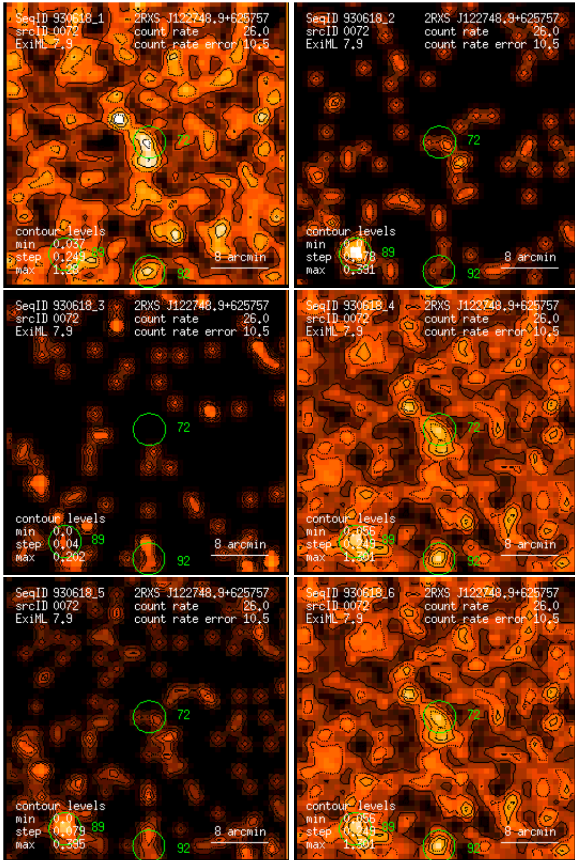
Figure 72: RASS 930618: detection 0072: band rate images, Gaussian filter: (1) PSPC channels 11 – 41, (2) 52 – 90, (3) 91 – 201, (4) 11 – 235, (5) 52 – 201, (6) 11 – 201. Broad band rates in counts/ks. Band rate contour levels in counts/ks/arcmin 2 .
