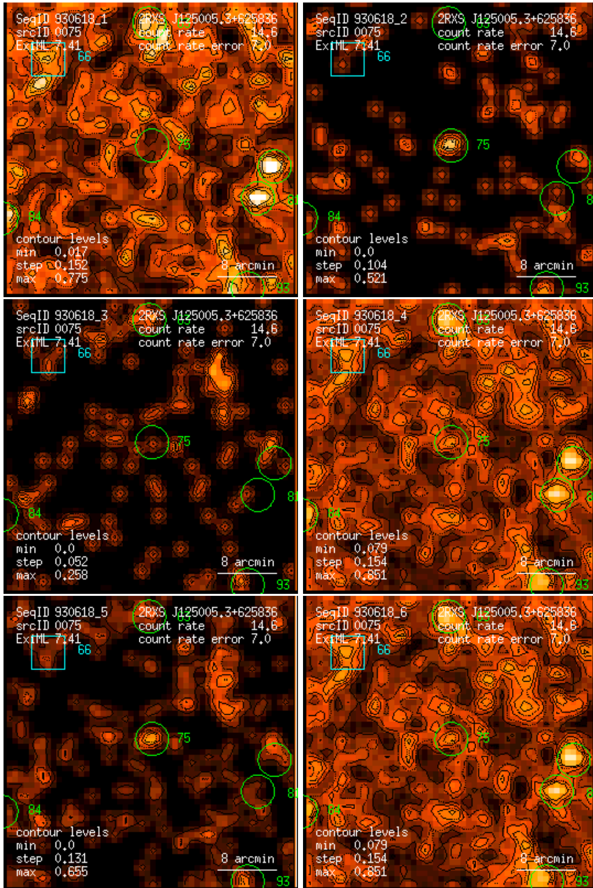
Figure 75: RASS 930618: detection 0075: band rate images, Gaussian filter: (1) PSPC channels 11 – 41, (2) 52 – 90, (3) 91 – 201, (4) 11 – 235, (5) 52 – 201, (6) 11 – 201. Broad band rates in counts/ks. Band rate contour levels in counts/ks/arcmin 2 .
