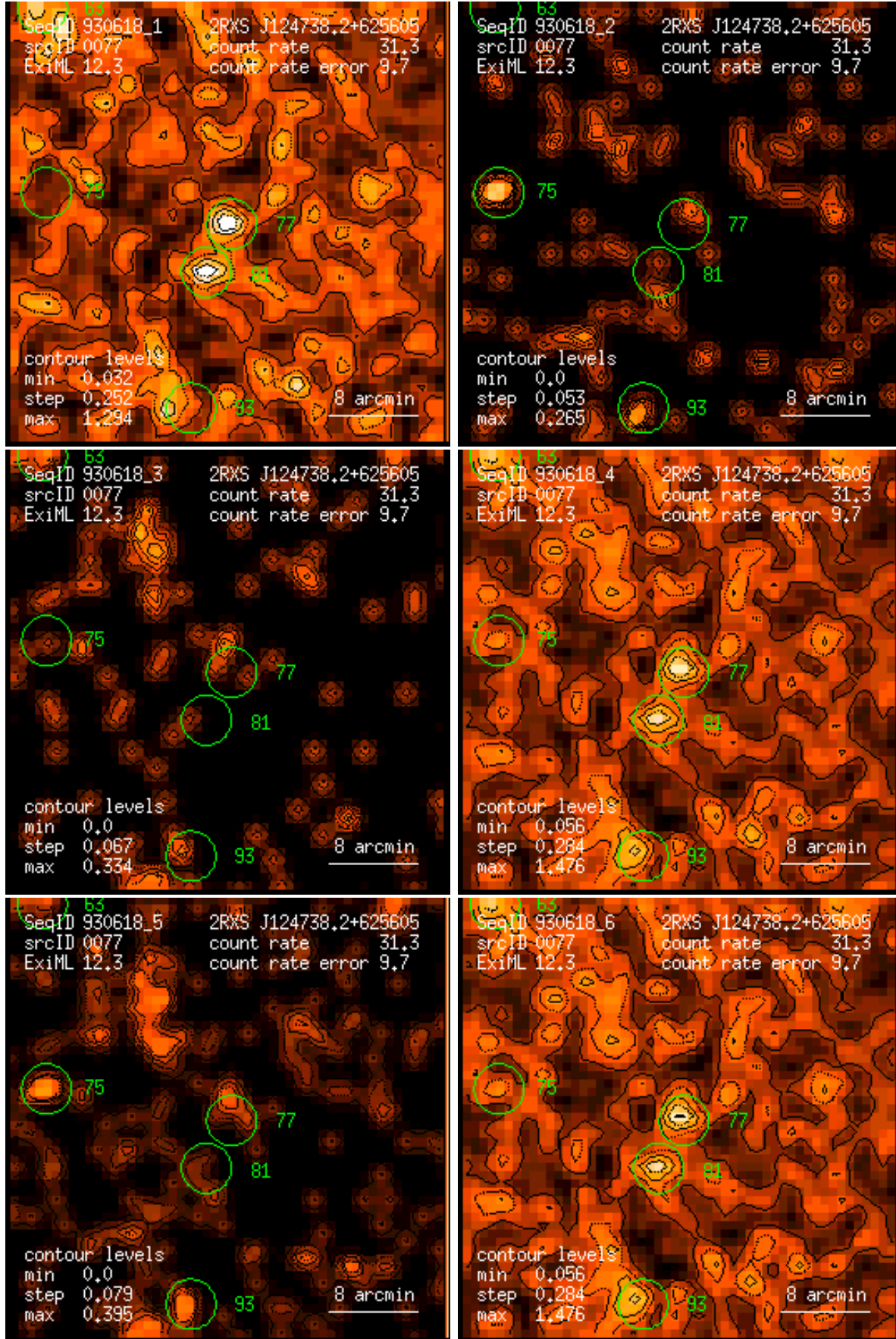
Figure 77: RASS 930618: detection 0077: band rate images, Gaussian filter: (1) PSPC channels 11 – 41, (2) 52 – 90, (3) 91 – 201, (4) 11 – 235, (5) 52 – 201, (6) 11 – 201. Broad band rates in counts/ks. Band rate contour levels in counts/ks/arcmin 2 .
