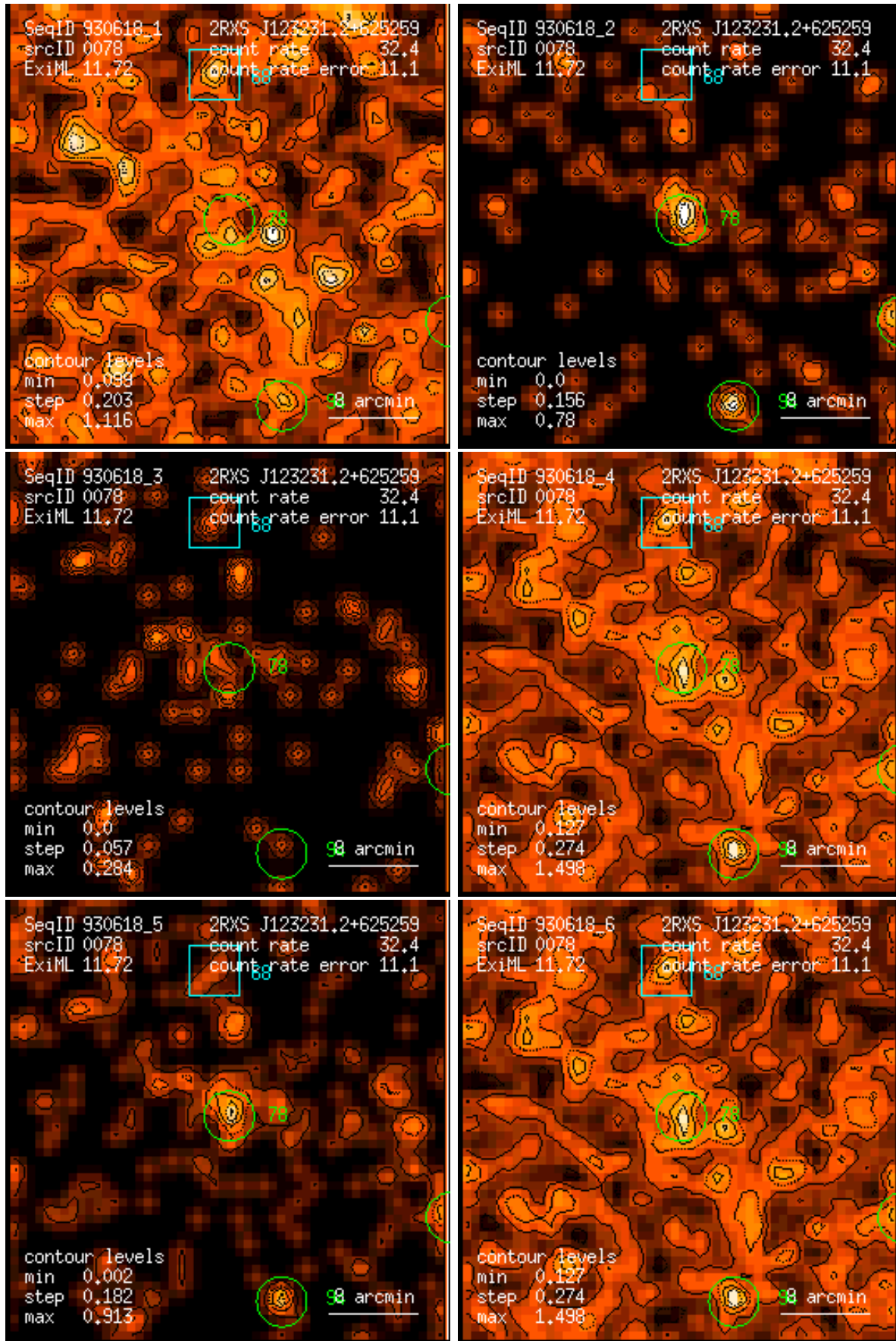
Figure 78: RASS 930618: detection 0078: band rate images, Gaussian filter: (1) PSPC channels 11 – 41, (2) 52 – 90, (3) 91 – 201, (4) 11 – 235, (5) 52 – 201, (6) 11 – 201. Broad band rates in counts/ks. Band rate contour levels in counts/ks/arcmin 2 .
