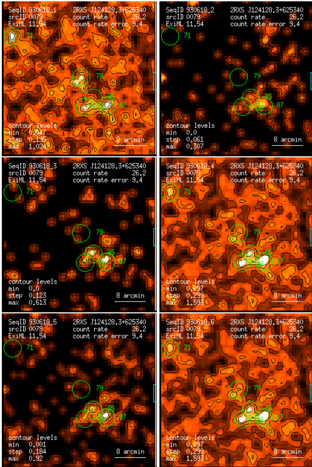
Figure 79: RASS 930618: detection 0079: band rate images, Gaussian filter: (1) PSPC channels 11 – 41, (2) 52 – 90, (3) 91 – 201, (4) 11 – 235, (5) 52 – 201, (6) 11 – 201. Broad band rates in counts/ks. Band rate contour levels in counts/ks/arcmin 2 .
