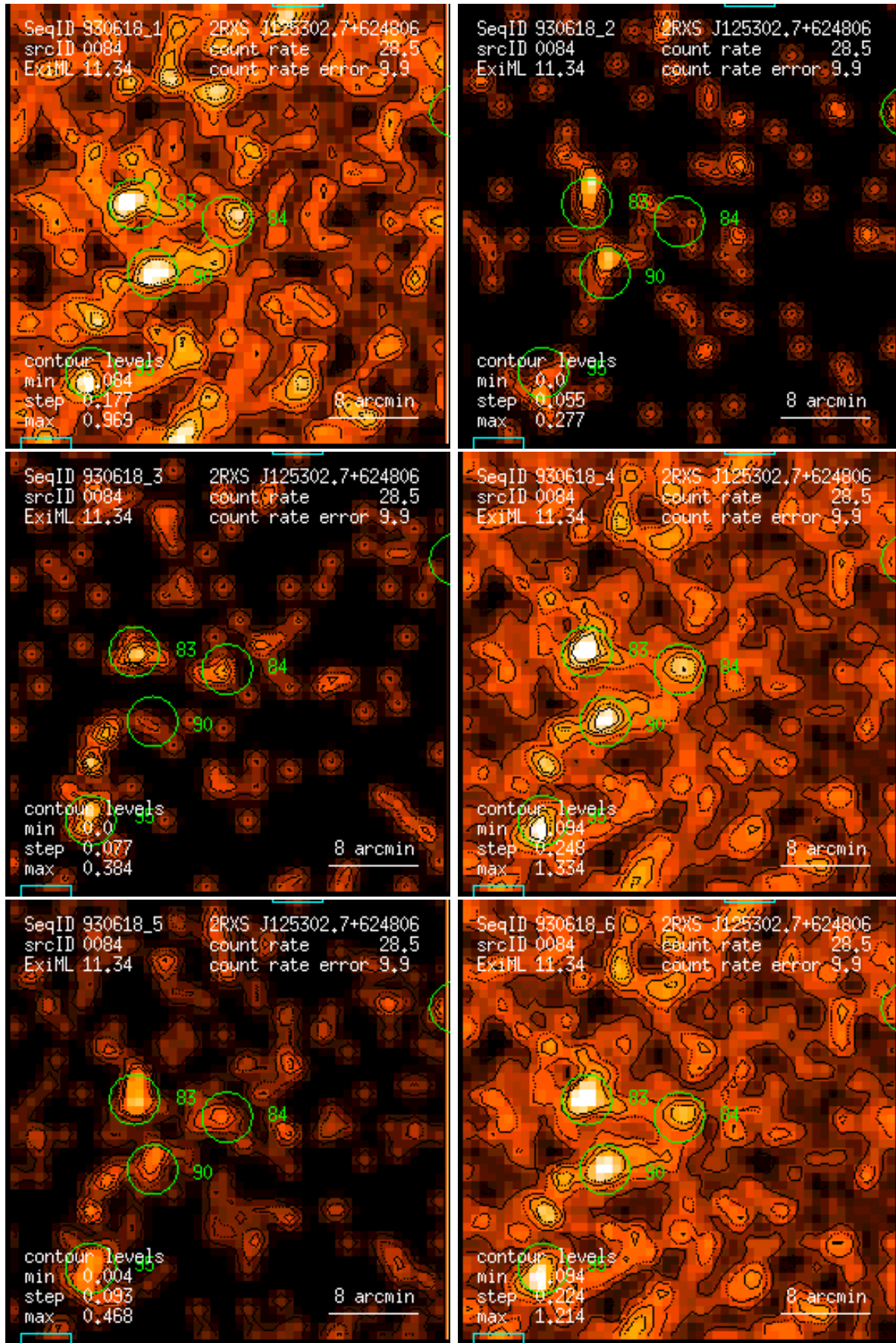
Figure 84: RASS 930618: detection 0084: band rate images, Gaussian filter: (1) PSPC channels 11 – 41, (2) 52 – 90, (3) 91 – 201, (4) 11 – 235, (5) 52 – 201, (6) 11 – 201. Broad band rates in counts/ks. Band rate contour levels in counts/ks/arcmin 2 .
