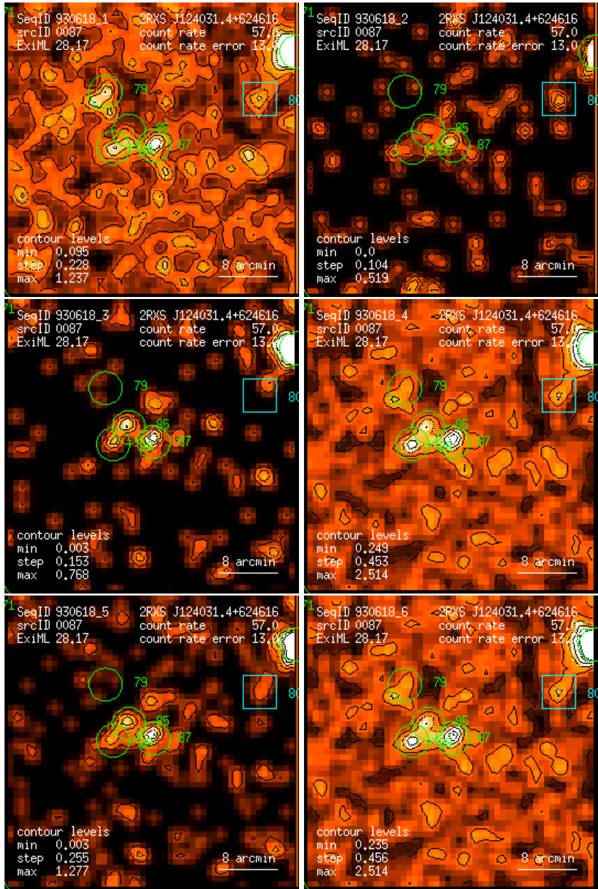
Figure 87: RASS 930618: detection 0087: band rate images, Gaussian filter: (1) PSPC channels 11 – 41, (2) 52 – 90, (3) 91 – 201, (4) 11 – 235, (5) 52 – 201, (6) 11 – 201. Broad band rates in counts/ks. Band rate contour levels in counts/ks/arcmin 2 .
