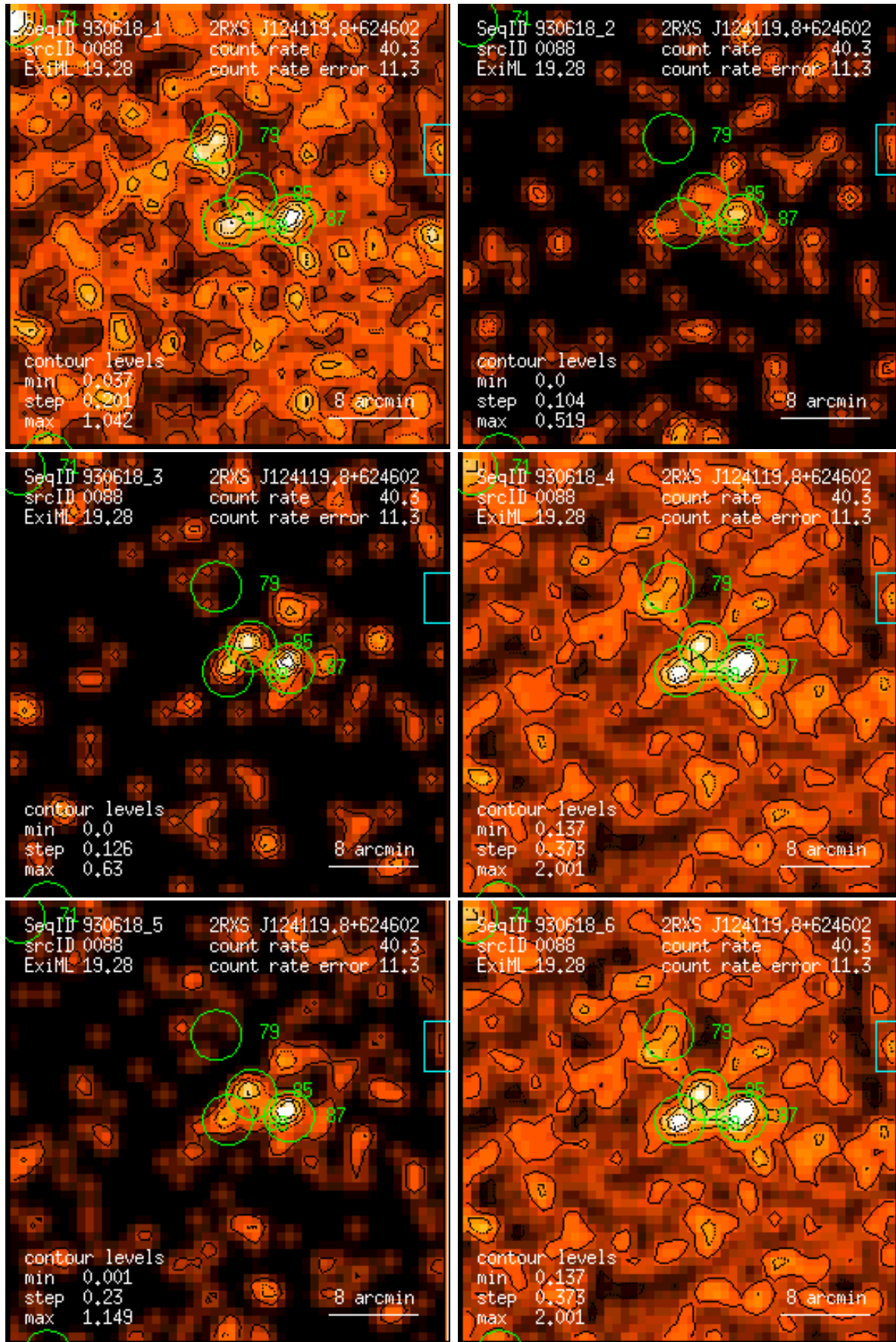
Figure 88: RASS 930618: detection 0088: band rate images, Gaussian filter: (1) PSPC channels 11 – 41, (2) 52 – 90, (3) 91 – 201, (4) 11 – 235, (5) 52 – 201, (6) 11 – 201. Broad band rates in counts/ks. Band rate contour levels in counts/ks/arcmin 2 .
