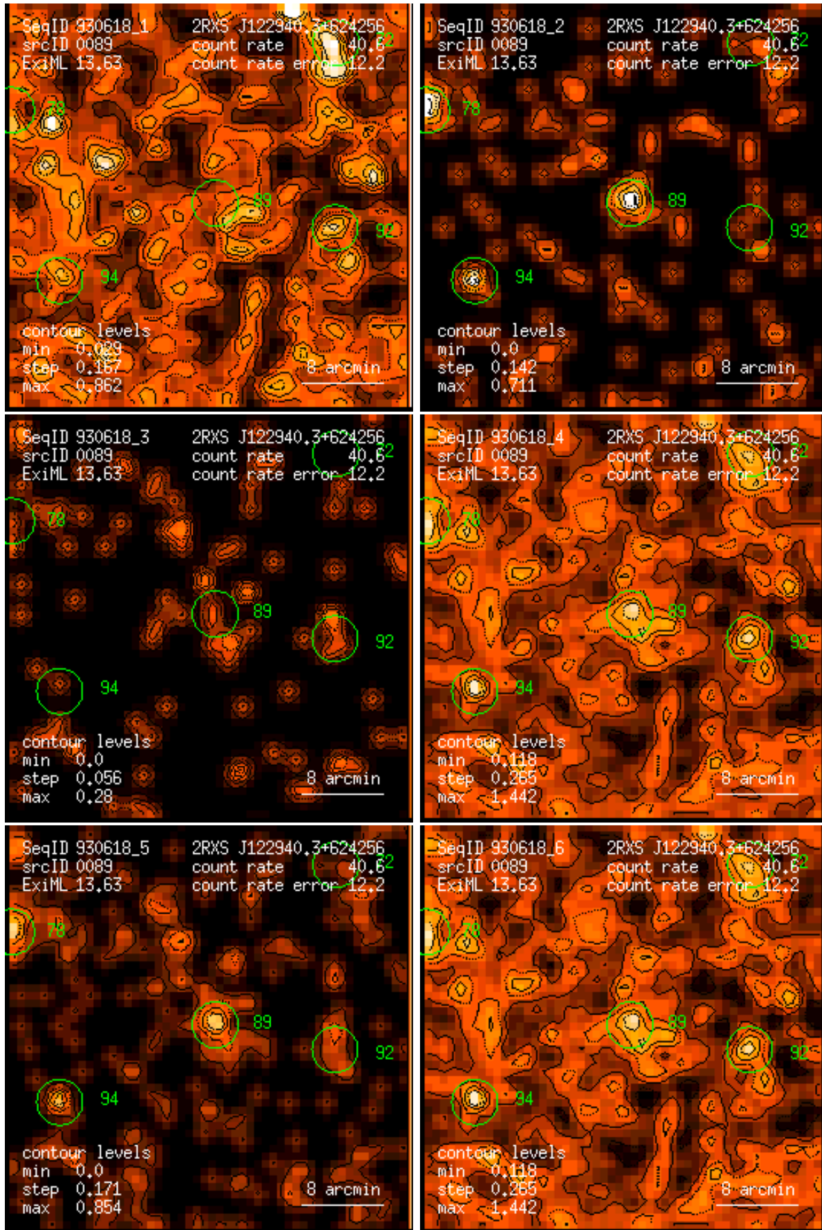
Figure 89: RASS 930618: detection 0089: band rate images, Gaussian filter: (1) PSPC channels 11 – 41, (2) 52 – 90, (3) 91 – 201, (4) 11 – 235, (5) 52 – 201, (6) 11 – 201. Broad band rates in counts/ks. Band rate contour levels in counts/ks/arcmin 2 .
