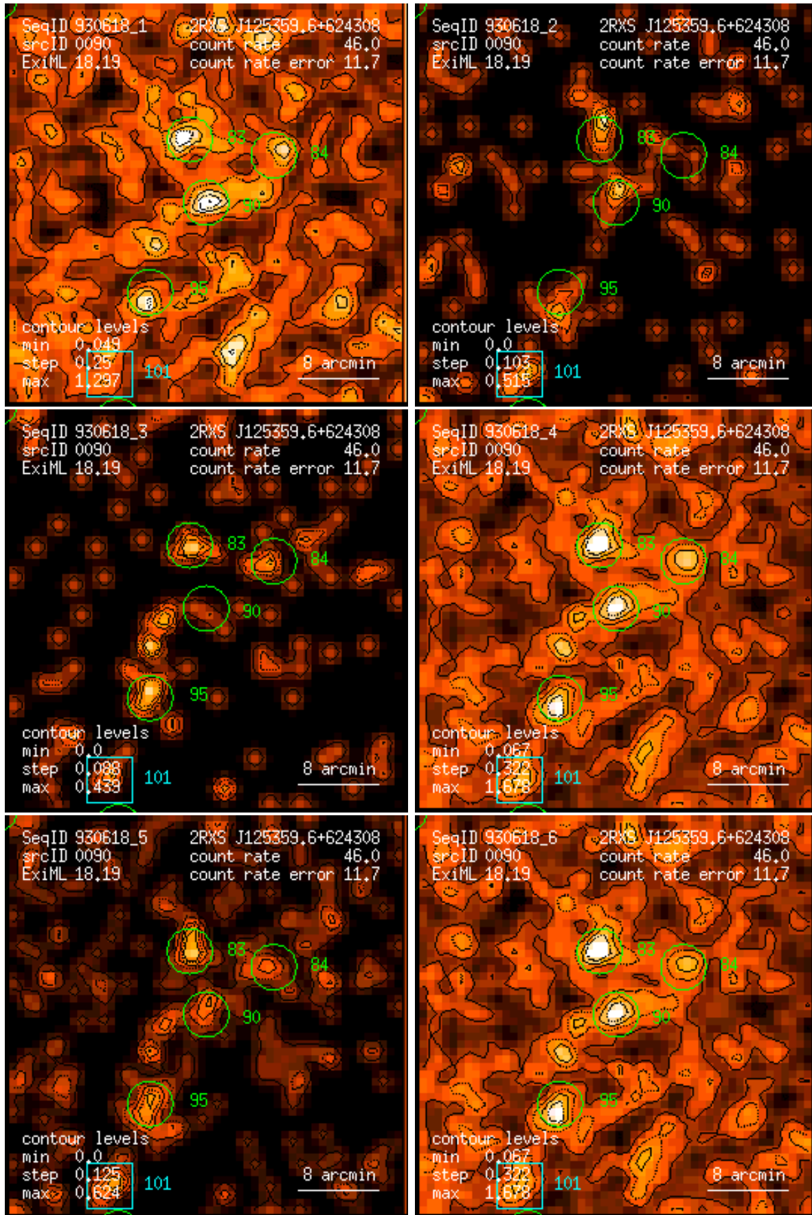
Figure 90: RASS 930618: detection 0090: band rate images, Gaussian filter: (1) PSPC channels 11 – 41, (2) 52 – 90, (3) 91 – 201, (4) 11 – 235, (5) 52 – 201, (6) 11 – 201. Broad band rates in counts/ks. Band rate contour levels in counts/ks/arcmin 2 .
