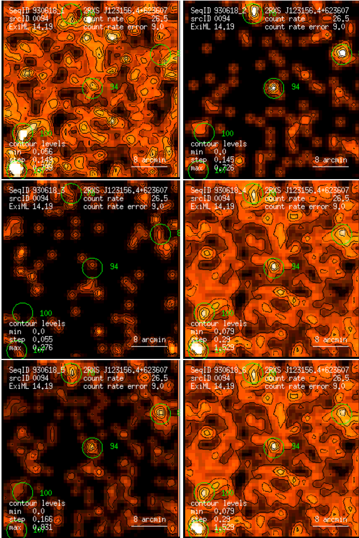
Figure 94: RASS 930618: detection 0094: band rate images, Gaussian filter: (1) PSPC channels 11 – 41, (2) 52 – 90, (3) 91 – 201, (4) 11 – 235, (5) 52 – 201, (6) 11 – 201. Broad band rates in counts/ks. Band rate contour levels in counts/ks/arcmin 2 .
