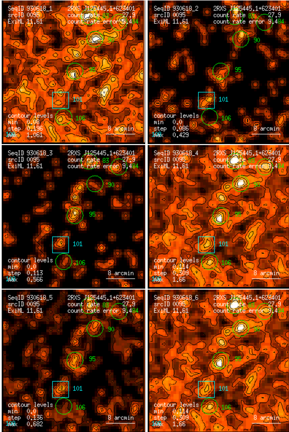
Figure 95: RASS 930618: detection 0095: band rate images, Gaussian filter: (1) PSPC channels 11 – 41, (2) 52 – 90, (3) 91 – 201, (4) 11 – 235, (5) 52 – 201, (6) 11 – 201. Broad band rates in counts/ks. Band rate contour levels in counts/ks/arcmin 2 .
