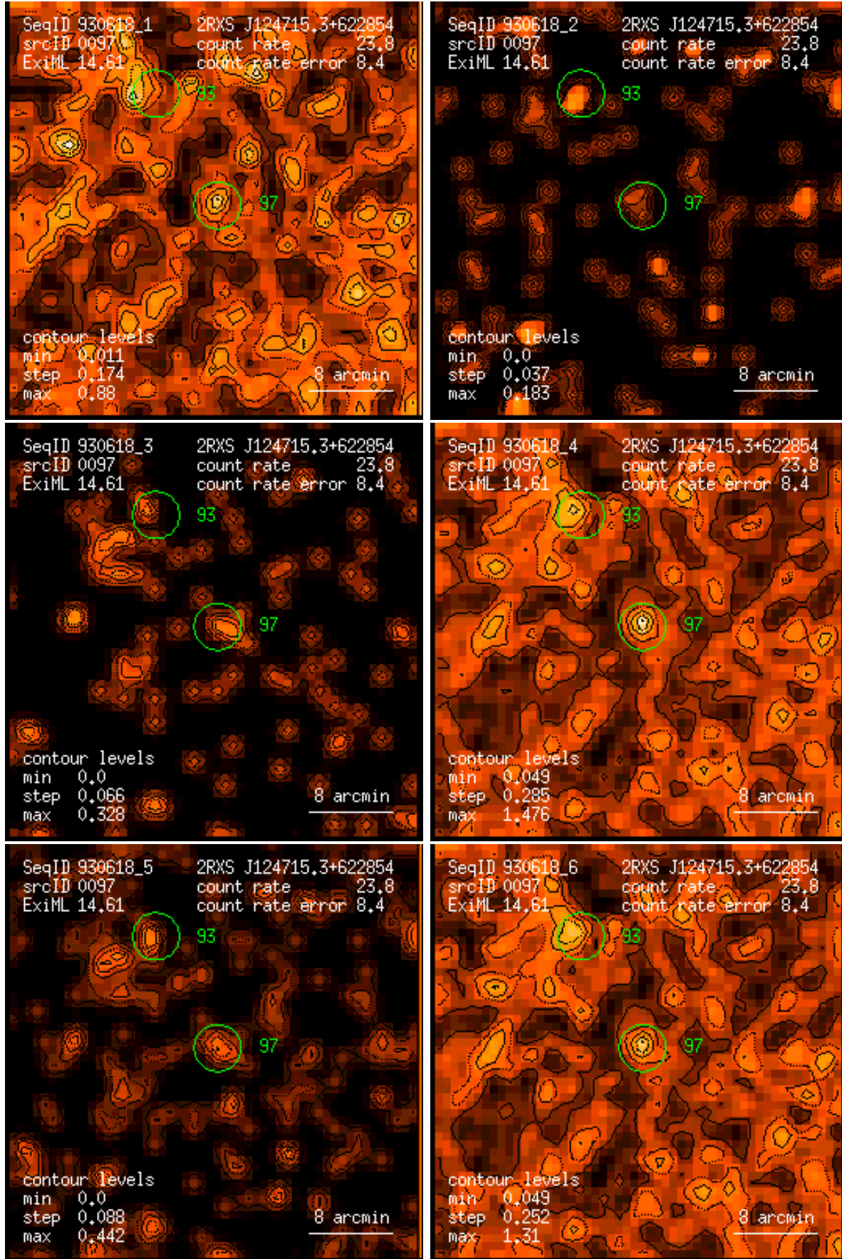
Figure 97: RASS 930618: detection 0097: band rate images, Gaussian filter: (1) PSPC channels 11 – 41, (2) 52 – 90, (3) 91 – 201, (4) 11 – 235, (5) 52 – 201, (6) 11 – 201. Broad band rates in counts/ks. Band rate contour levels in counts/ks/arcmin 2 .
