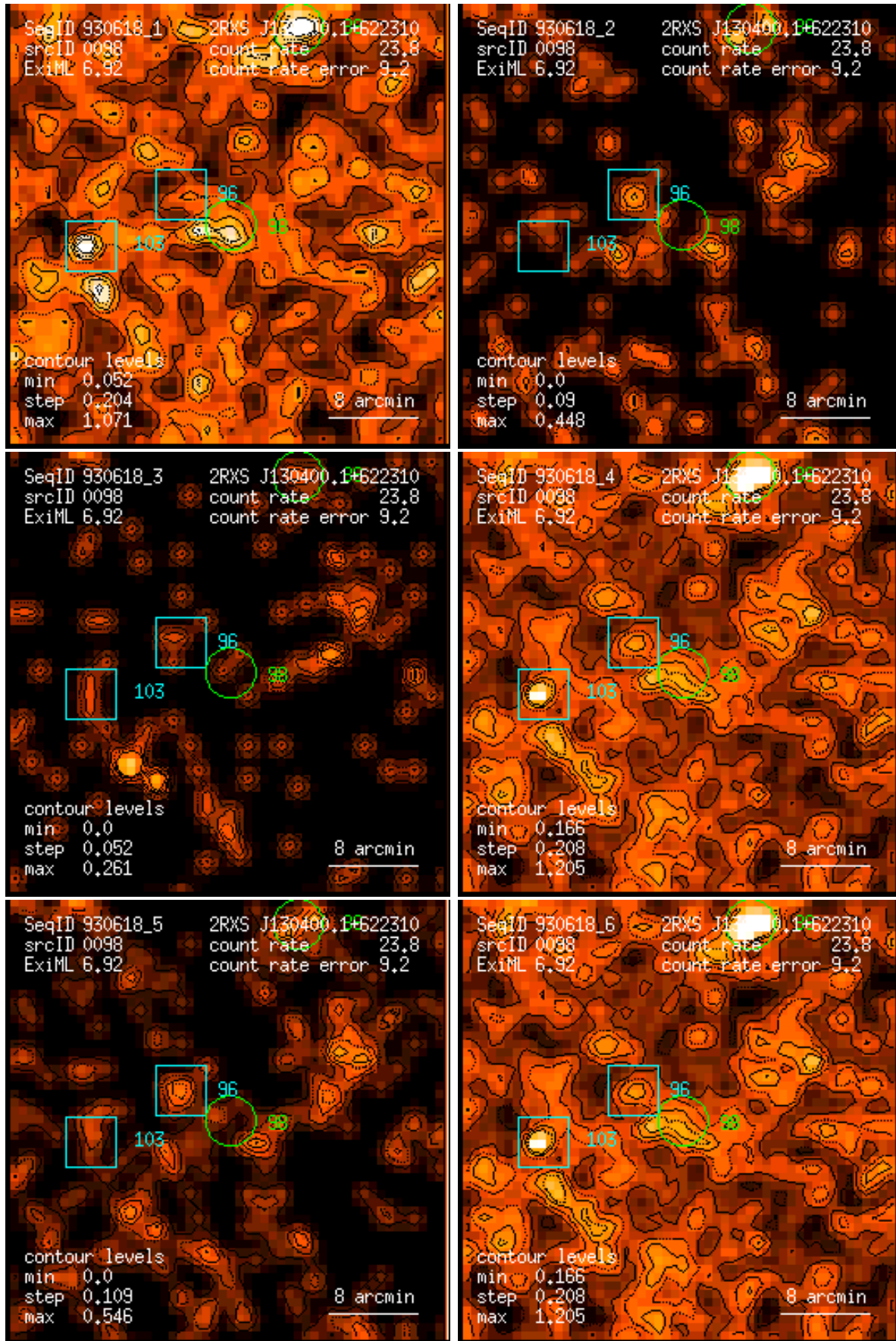
Figure 98: RASS 930618: detection 0098: band rate images, Gaussian filter: (1) PSPC channels 11 – 41, (2) 52 – 90, (3) 91 – 201, (4) 11 – 235, (5) 52 – 201, (6) 11 – 201. Broad band rates in counts/ks. Band rate contour levels in counts/ks/arcmin 2 .
