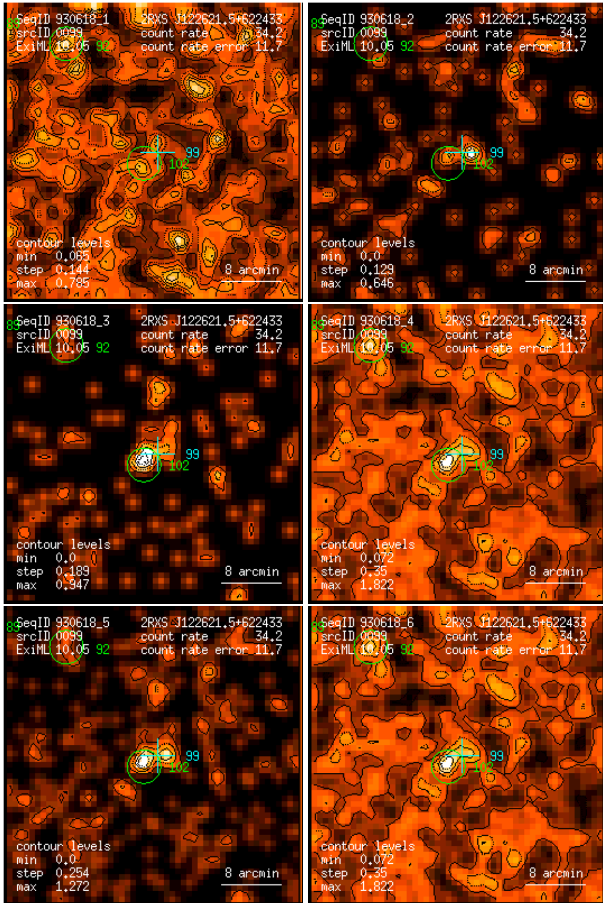
Figure 99: RASS 930618: detection 0099: band rate images, Gaussian filter: (1) PSPC channels 11 – 41, (2) 52 – 90, (3) 91 – 201, (4) 11 – 235, (5) 52 – 201, (6) 11 – 201. Broad band rates in counts/ks. Band rate contour levels in counts/ks/arcmin 2 .
