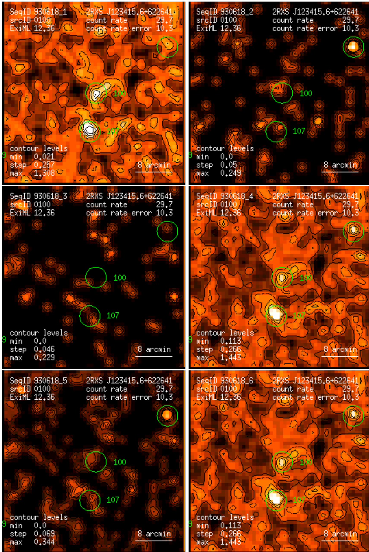
Figure 100: RASS 930618: detection 0100: band rate images, Gaussian filter: (1) PSPC channels 11 – 41, (2) 52 – 90, (3) 91 – 201, (4) 11 – 235, (5) 52 – 201, (6) 11 – 201. Broad band rates in counts/ks. Band rate contour levels in counts/ks/arcmin 2 .
