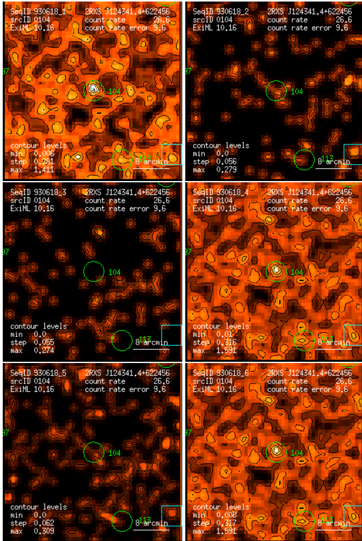
Figure 104: RASS 930618: detection 0104: band rate images, Gaussian filter: (1) PSPC channels 11 – 41, (2) 52 – 90, (3) 91 – 201, (4) 11 – 235, (5) 52 – 201, (6) 11 – 201. Broad band rates in counts/ks. Band rate contour levels in counts/ks/arcmin 2 .
