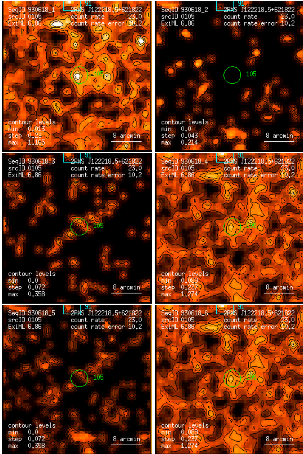
Figure 105: RASS 930618: detection 0105: band rate images, Gaussian filter: (1) PSPC channels 11 – 41, (2) 52 – 90, (3) 91 – 201, (4) 11 – 235, (5) 52 – 201, (6) 11 – 201. Broad band rates in counts/ks. Band rate contour levels in counts/ks/arcmin 2 .
