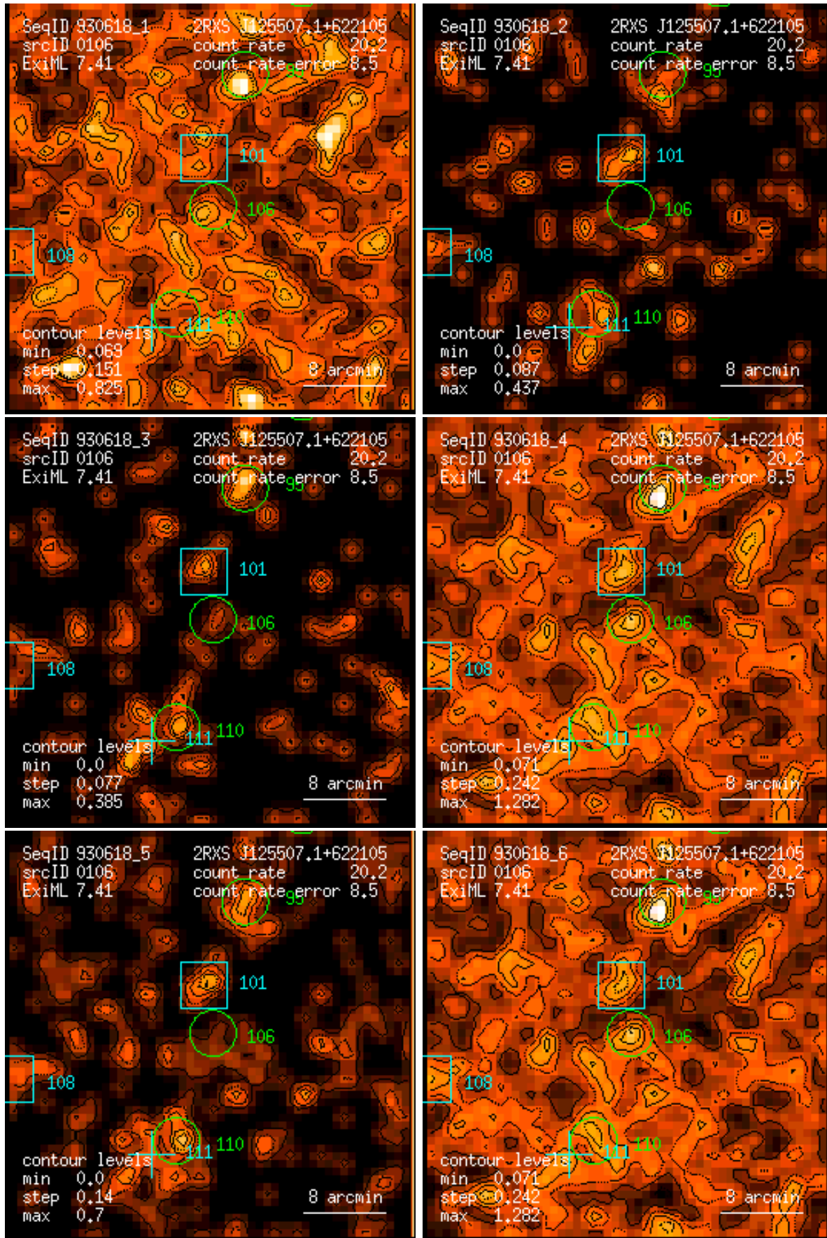
Figure 106: RASS 930618: detection 0106: band rate images, Gaussian filter: (1) PSPC channels 11 – 41, (2) 52 – 90, (3) 91 – 201, (4) 11 – 235, (5) 52 – 201, (6) 11 – 201. Broad band rates in counts/ks. Band rate contour levels in counts/ks/arcmin 2 .
