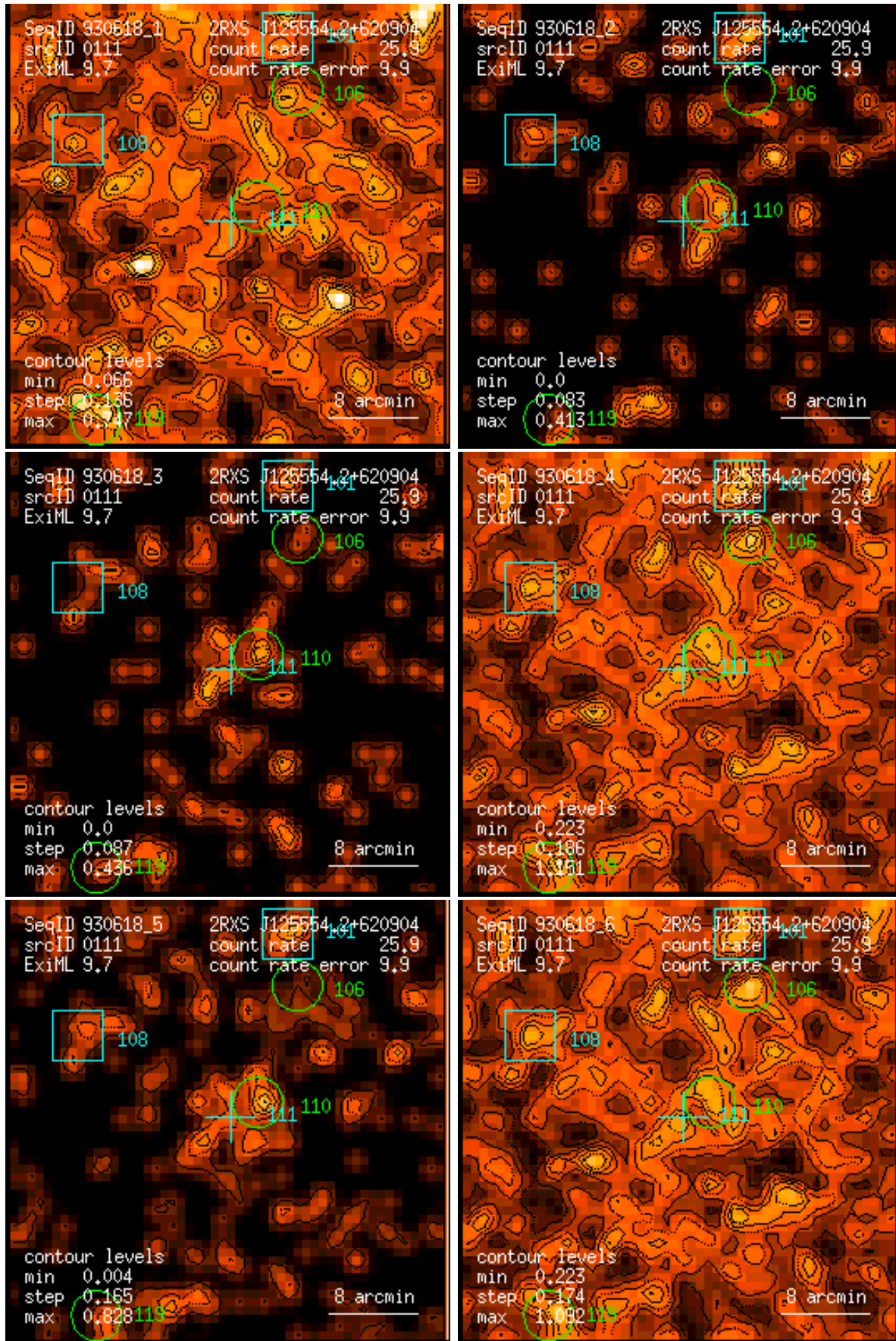
Figure 111: RASS 930618: detection 0111: band rate images, Gaussian filter: (1) PSPC channels 11 – 41, (2) 52 – 90, (3) 91 – 201, (4) 11 – 235, (5) 52 – 201, (6) 11 – 201. Broad band rates in counts/ks. Band rate contour levels in counts/ks/arcmin 2 .
