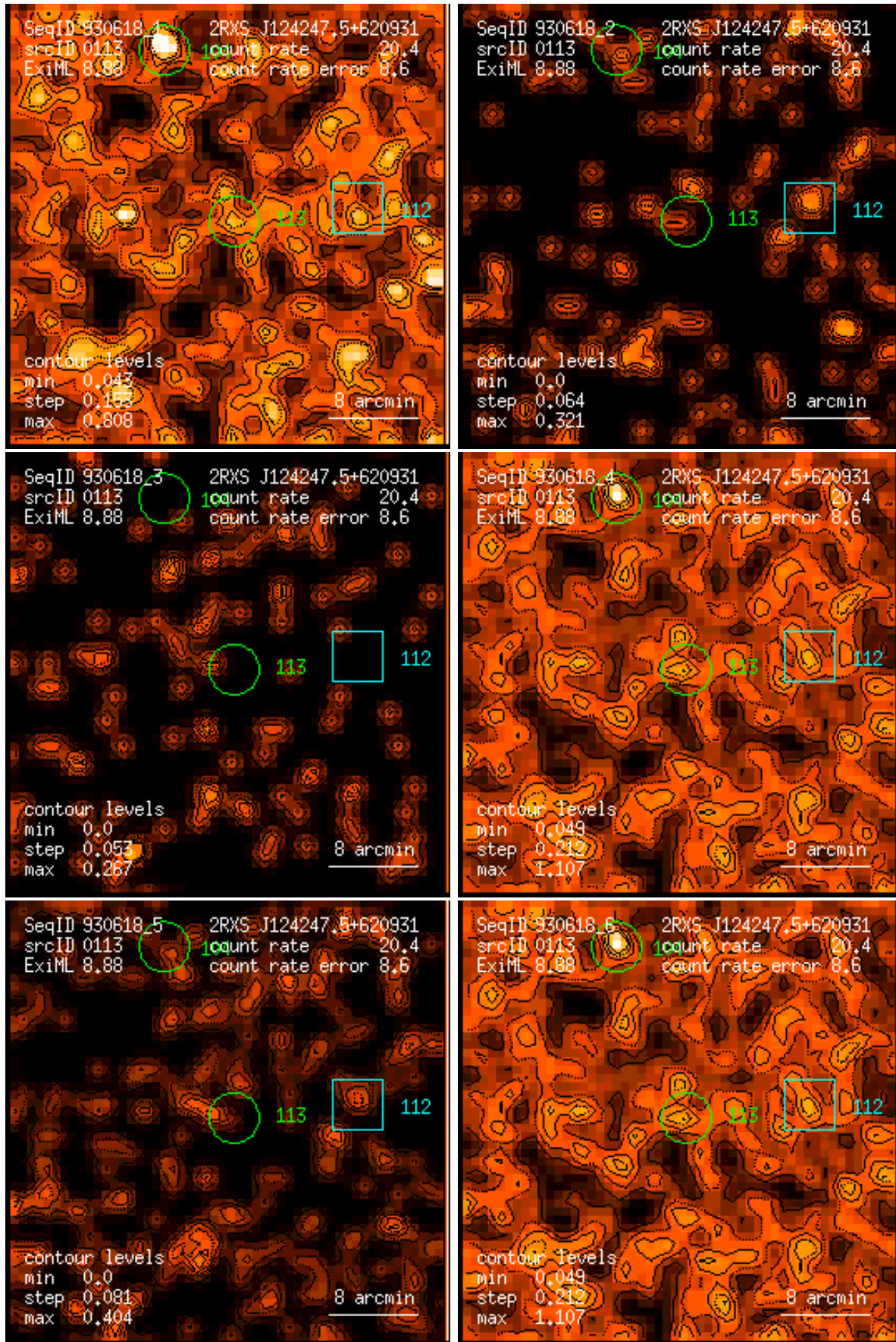
Figure 113: RASS 930618: detection 0113: band rate images, Gaussian filter: (1) PSPC channels 11 – 41, (2) 52 – 90, (3) 91 – 201, (4) 11 – 235, (5) 52 – 201, (6) 11 – 201. Broad band rates in counts/ks. Band rate contour levels in counts/ks/arcmin 2 .
