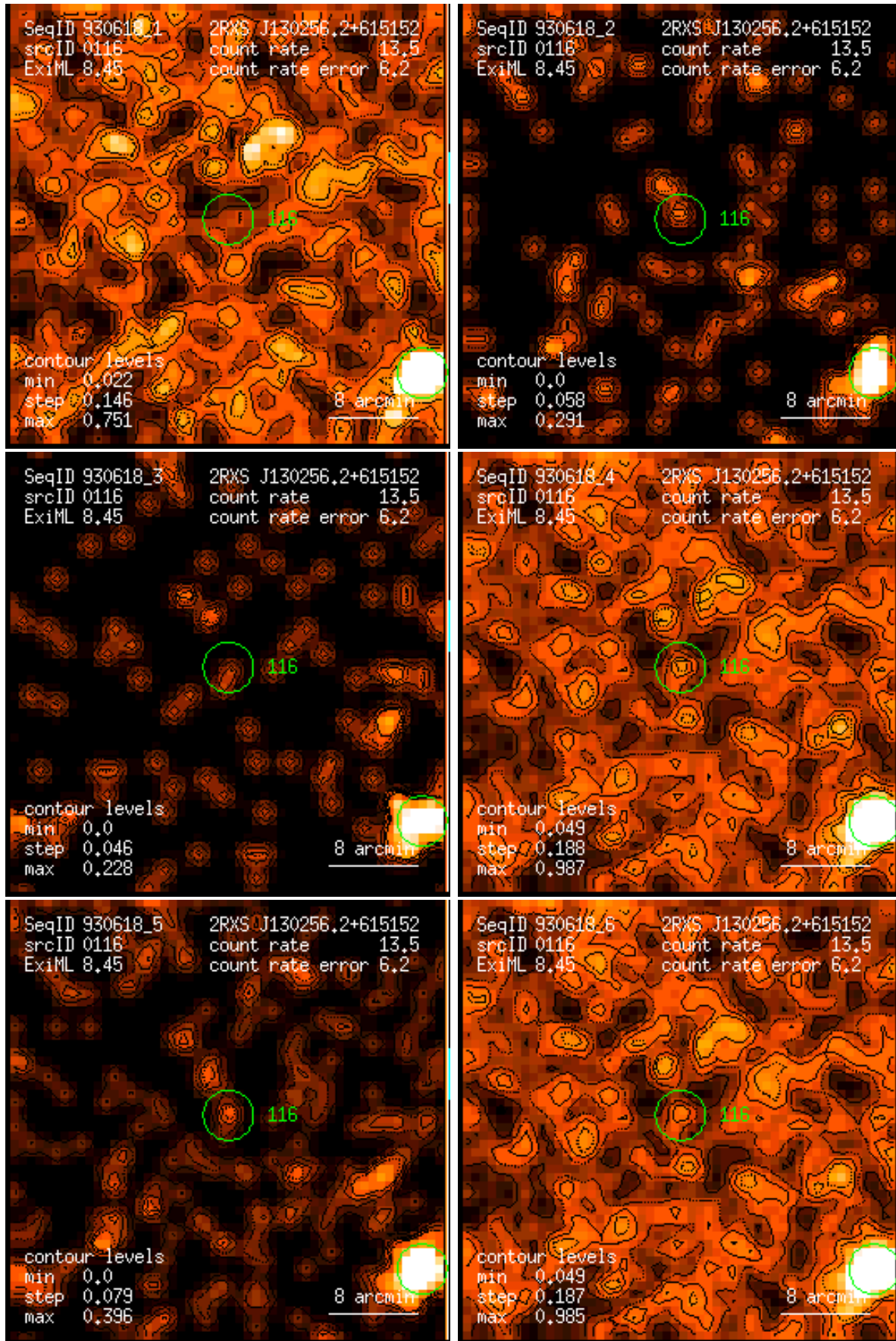
Figure 116: RASS 930618: detection 0116: band rate images, Gaussian filter: (1) PSPC channels 11 – 41, (2) 52 – 90, (3) 91 – 201, (4) 11 – 235, (5) 52 – 201, (6) 11 – 201. Broad band rates in counts/ks. Band rate contour levels in counts/ks/arcmin 2 .
