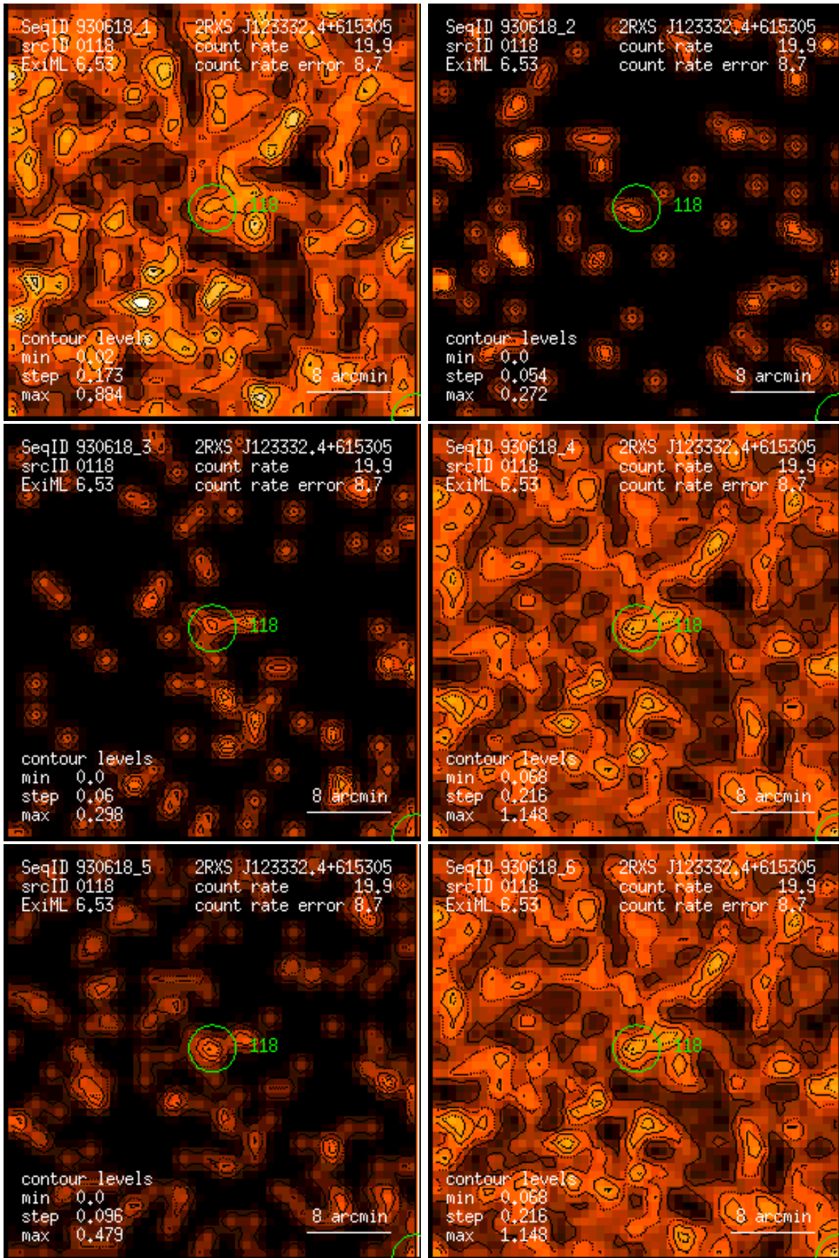
Figure 118: RASS 930618: detection 0118: band rate images, Gaussian filter: (1) PSPC channels 11 – 41, (2) 52 – 90, (3) 91 – 201, (4) 11 – 235, (5) 52 – 201, (6) 11 – 201. Broad band rates in counts/ks. Band rate contour levels in counts/ks/arcmin 2 .
