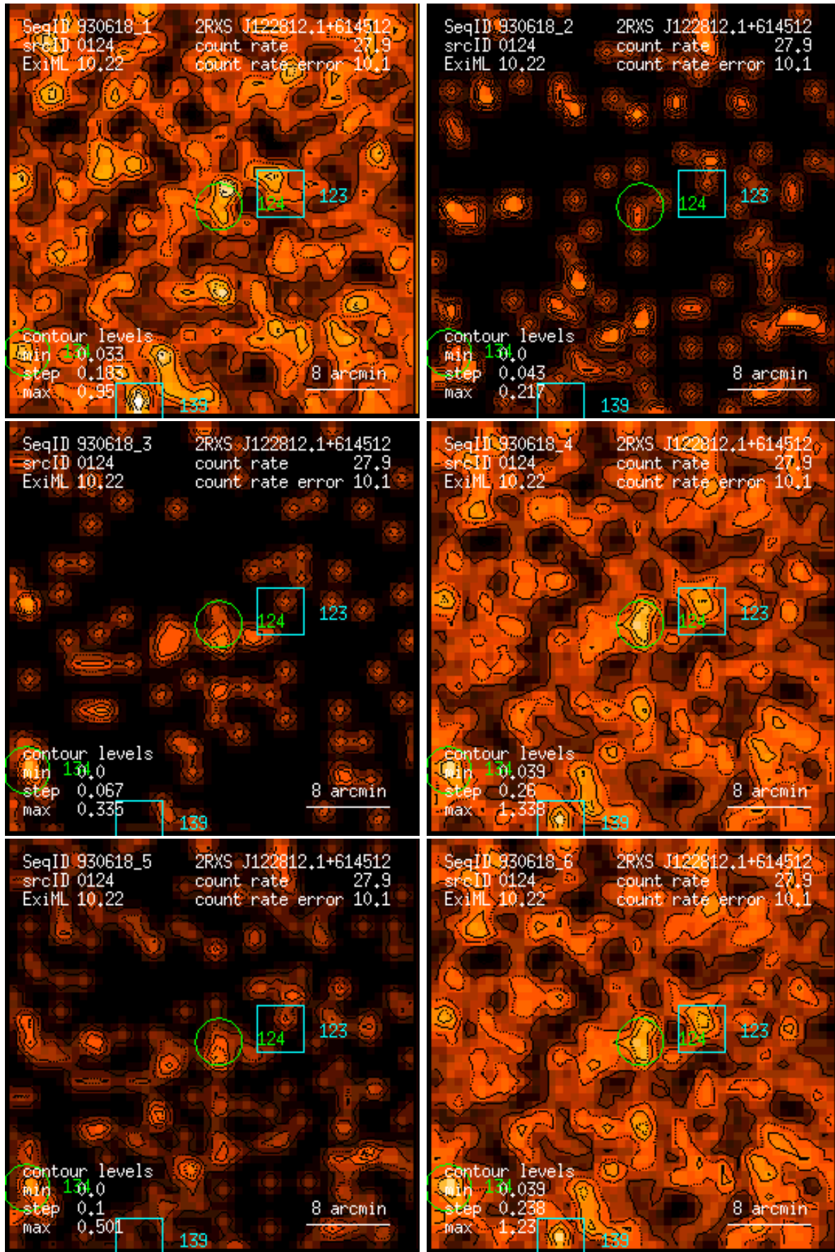
Figure 124: RASS 930618: detection 0124: band rate images, Gaussian filter: (1) PSPC channels 11 – 41, (2) 52 – 90, (3) 91 – 201, (4) 11 – 235, (5) 52 – 201, (6) 11 – 201. Broad band rates in counts/ks. Band rate contour levels in counts/ks/arcmin 2 .
